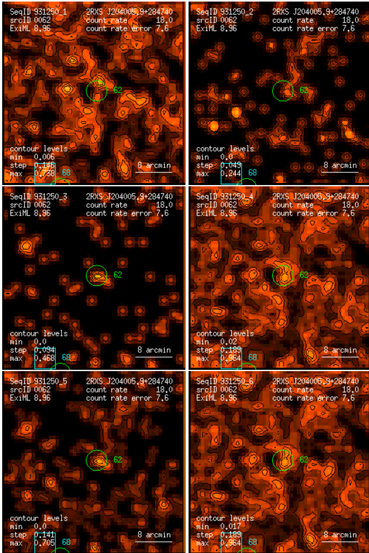
Figure 62: RASS 931250: detection 0062: band rate images, Gaussian filter: (1) PSPC channels 11 – 41, (2) 52 – 90, (3) 91 – 201, (4) 11 – 235, (5) 52 – 201, (6) 11 – 201. Broad band rates in counts/ks. Band rate contour levels in counts/ks/arcmin 2 .
