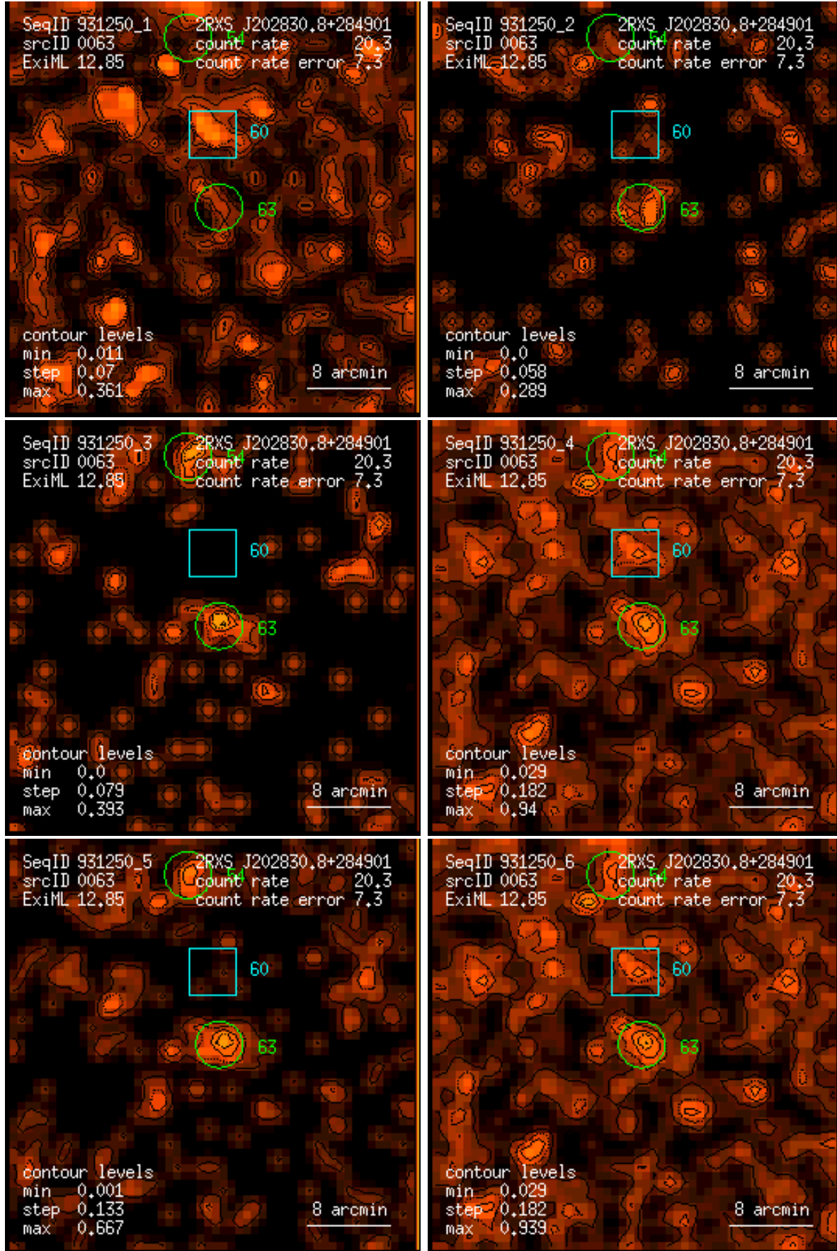
Figure 63: RASS 931250: detection 0063: band rate images, Gaussian filter: (1) PSPC channels 11 – 41, (2) 52 – 90, (3) 91 – 201, (4) 11 – 235, (5) 52 – 201, (6) 11 – 201. Broad band rates in counts/ks. Band rate contour levels in counts/ks/arcmin 2 .
