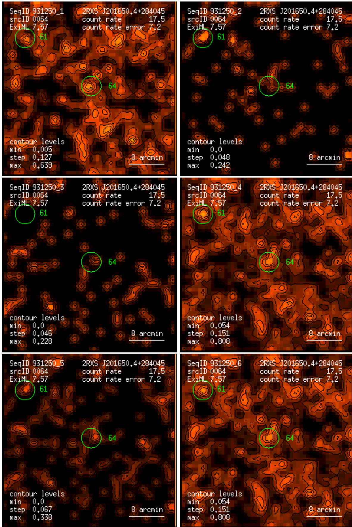
Figure 64: RASS 931250: detection 0064: band rate images, Gaussian filter: (1) PSPC channels 11 – 41, (2) 52 – 90, (3) 91 – 201, (4) 11 – 235, (5) 52 – 201, (6) 11 – 201. Broad band rates in counts/ks. Band rate contour levels in counts/ks/arcmin 2 .
