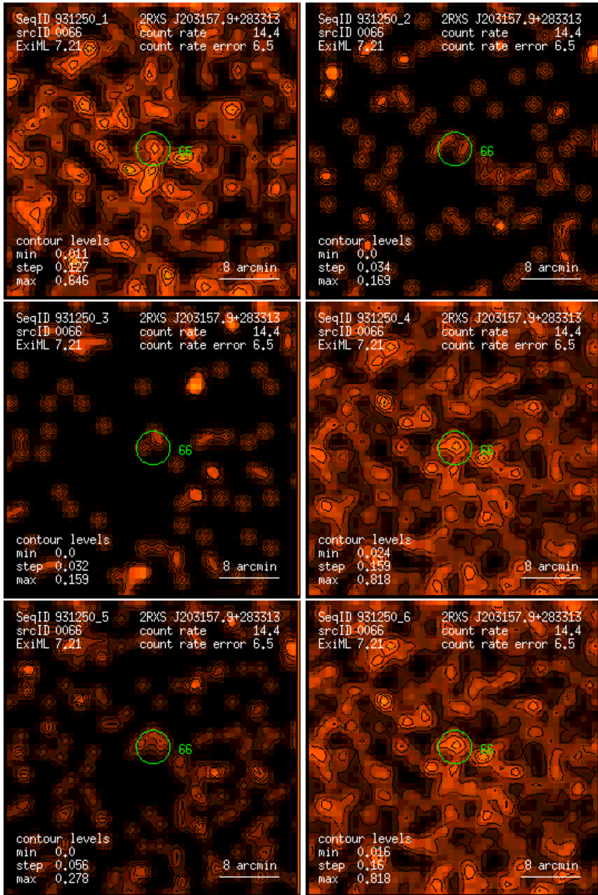
Figure 66: RASS 931250: detection 0066: band rate images, Gaussian filter: (1) PSPC channels 11 – 41, (2) 52 – 90, (3) 91 – 201, (4) 11 – 235, (5) 52 – 201, (6) 11 – 201. Broad band rates in counts/ks. Band rate contour levels in counts/ks/arcmin 2 .
