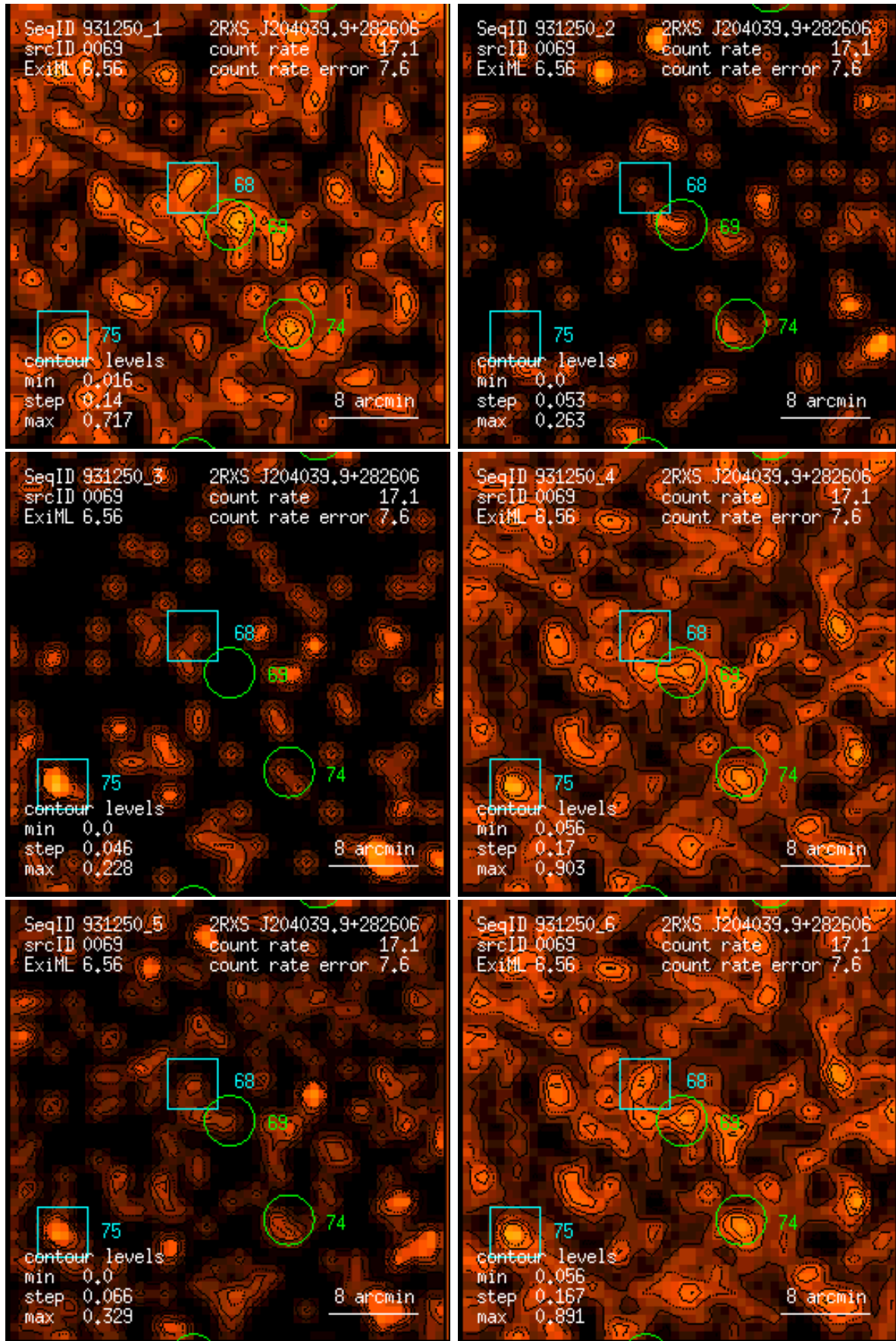
Figure 69: RASS 931250: detection 0069: band rate images, Gaussian filter: (1) PSPC channels 11 – 41, (2) 52 – 90, (3) 91 – 201, (4) 11 – 235, (5) 52 – 201, (6) 11 – 201. Broad band rates in counts/ks. Band rate contour levels in counts/ks/arcmin 2 .
