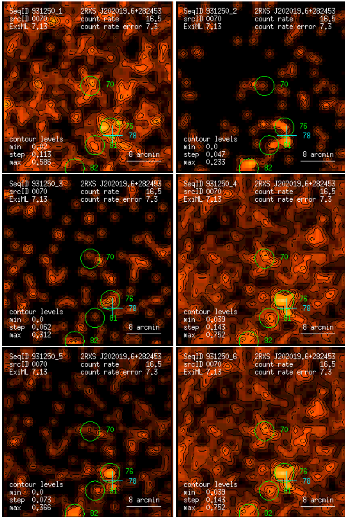
Figure 70: RASS 931250: detection 0070: band rate images, Gaussian filter: (1) PSPC channels 11 – 41, (2) 52 – 90, (3) 91 – 201, (4) 11 – 235, (5) 52 – 201, (6) 11 – 201. Broad band rates in counts/ks. Band rate contour levels in counts/ks/arcmin 2 .
