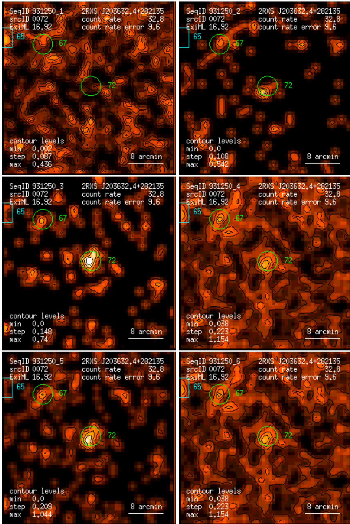
Figure 72: RASS 931250: detection 0072: band rate images, Gaussian filter: (1) PSPC channels 11 – 41, (2) 52 – 90, (3) 91 – 201, (4) 11 – 235, (5) 52 – 201, (6) 11 – 201. Broad band rates in counts/ks. Band rate contour levels in counts/ks/arcmin 2 .
