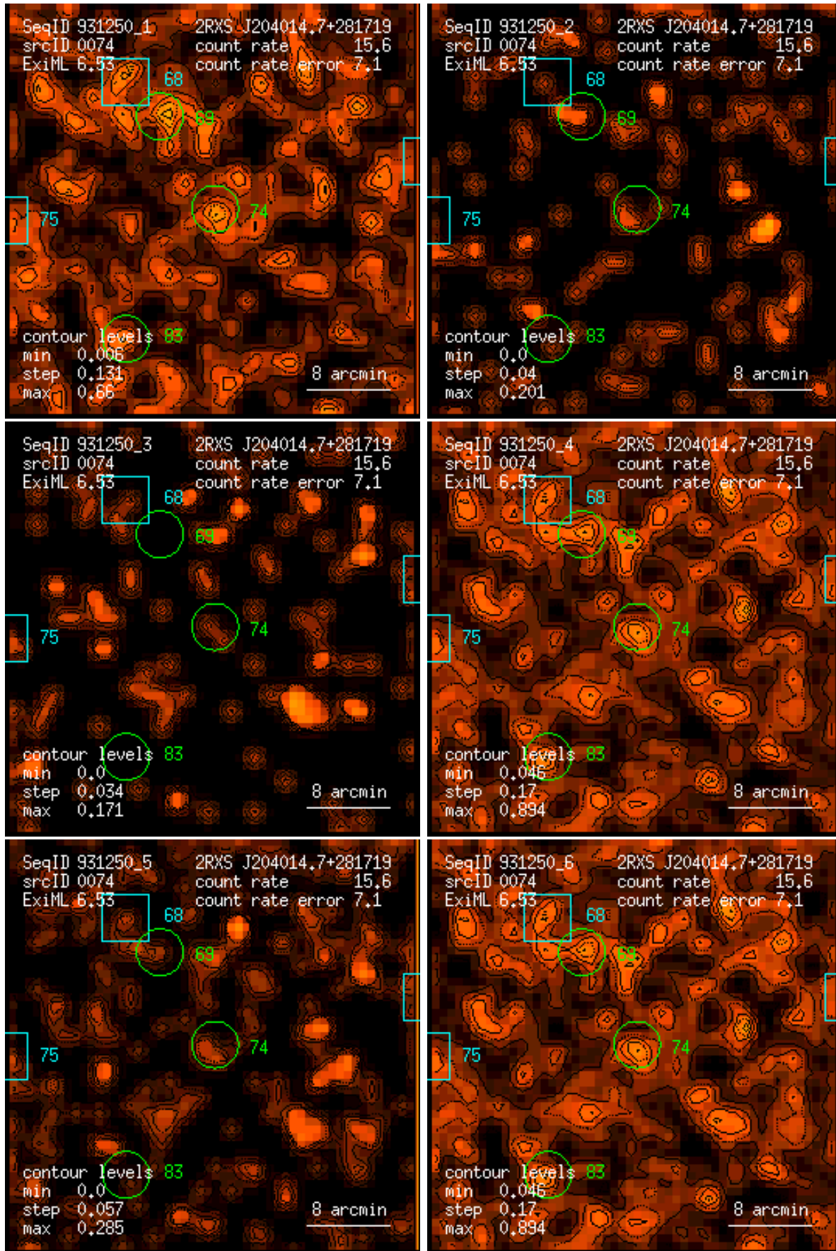
Figure 74: RASS 931250: detection 0074: band rate images, Gaussian filter: (1) PSPC channels 11 – 41, (2) 52 – 90, (3) 91 – 201, (4) 11 – 235, (5) 52 – 201, (6) 11 – 201. Broad band rates in counts/ks. Band rate contour levels in counts/ks/arcmin 2 .
