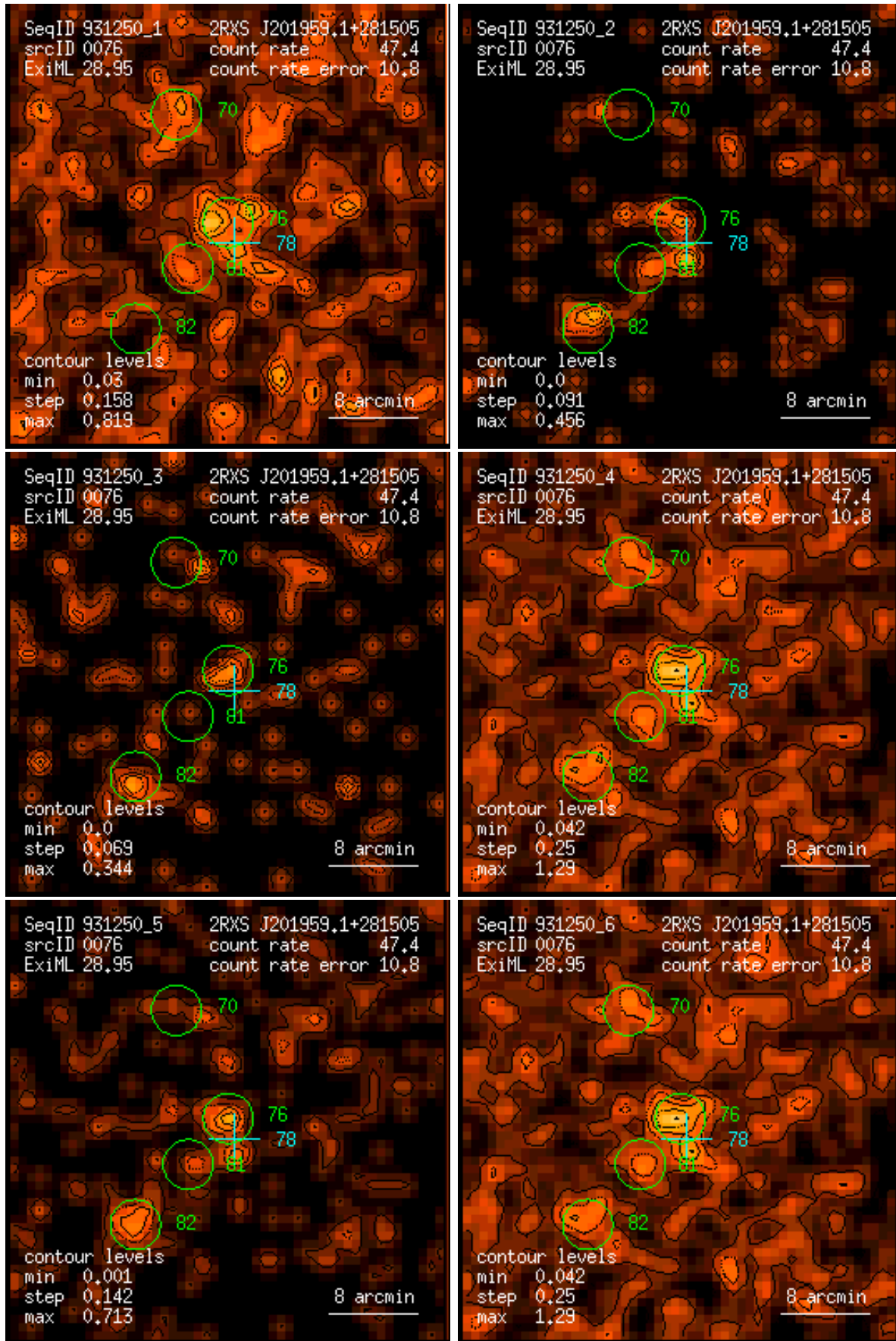
Figure 76: RASS 931250: detection 0076: band rate images, Gaussian filter: (1) PSPP channels 11 – 41, (2) 52 – 90, (3) 91 – 201, (4) 11 – 235, (5) 52 – 201, (6) 11 – 201. Broad band rates in counts/ks. Band rate contour levels in counts/ks/arcmin 2 .
