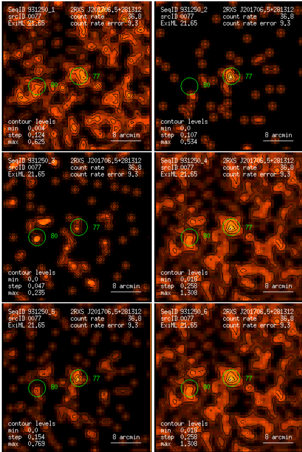
Figure 77: RASS 931250: detection 0077: band rate images, Gaussian filter: (1) PSPC channels 11 – 41, (2) 52 – 90, (3) 91 – 201, (4) 11 – 235, (5) 52 – 201, (6) 11 – 201. Broad band rates in counts/ks. Band rate contour levels in counts/ks/arcmin 2 .
