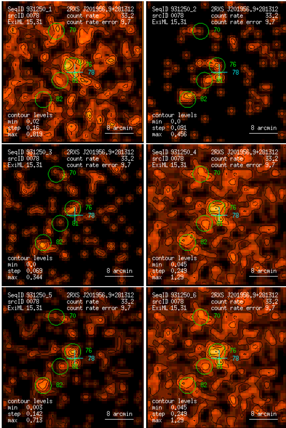
Figure 78: RASS 931250: detection 0078: band rate images, Gaussian filter: (1) PSPC channels 11 – 41, (2) 52 – 90, (3) 91 – 201, (4) 11 – 235, (5) 52 – 201, (6) 11 – 201. Broad band rates in counts/ks. Band rate contour levels in counts/ks/arcmin 2 .
