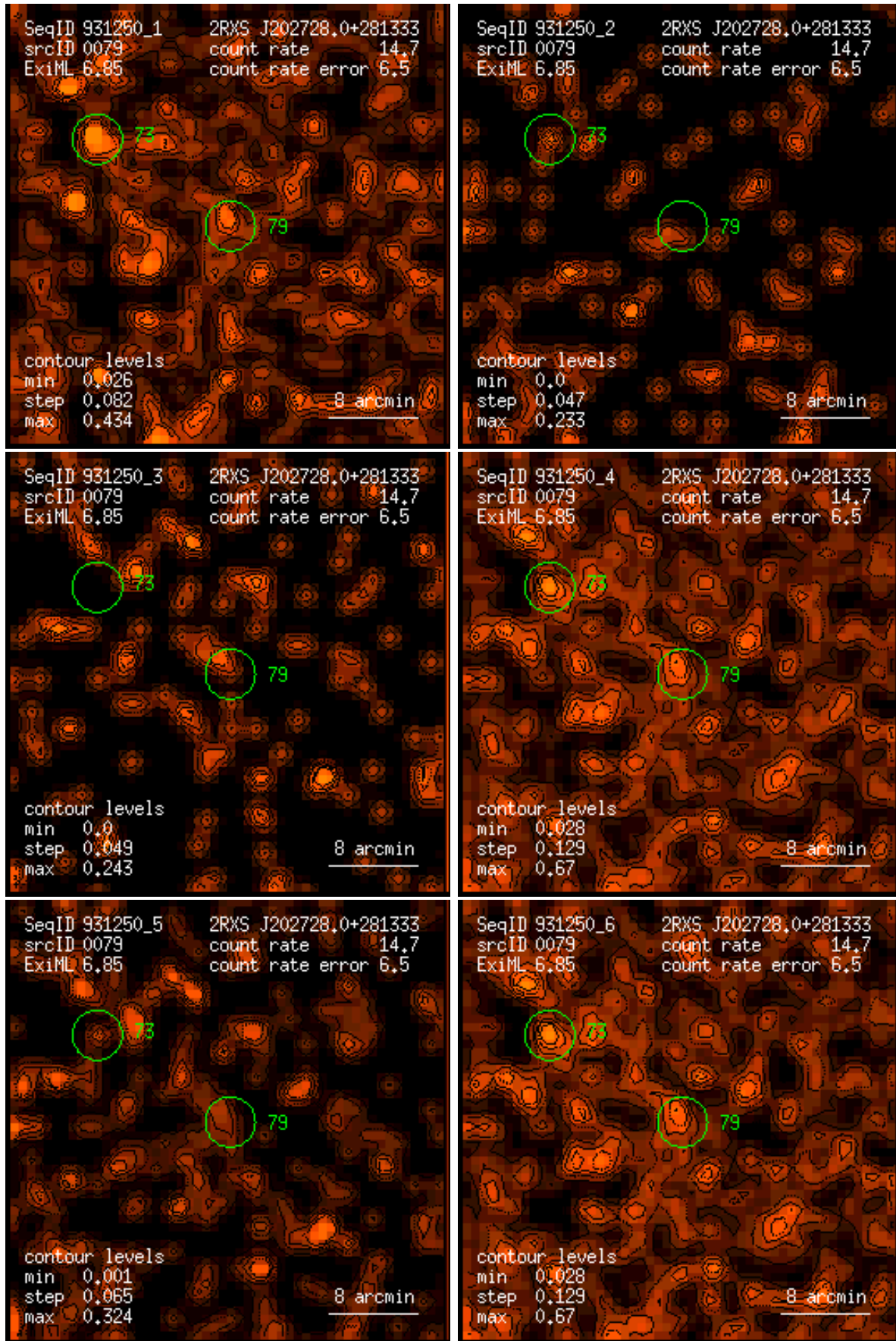
Figure 79: RASS 931250: detection 0079: band rate images, Gaussian filter: (1) PSPC channels 11 – 41, (2) 52 – 90, (3) 91 – 201, (4) 11 – 235, (5) 52 – 201, (6) 11 – 201. Broad band rates in counts/ks. Band rate contour levels in counts/ks/arcmin 2 .
