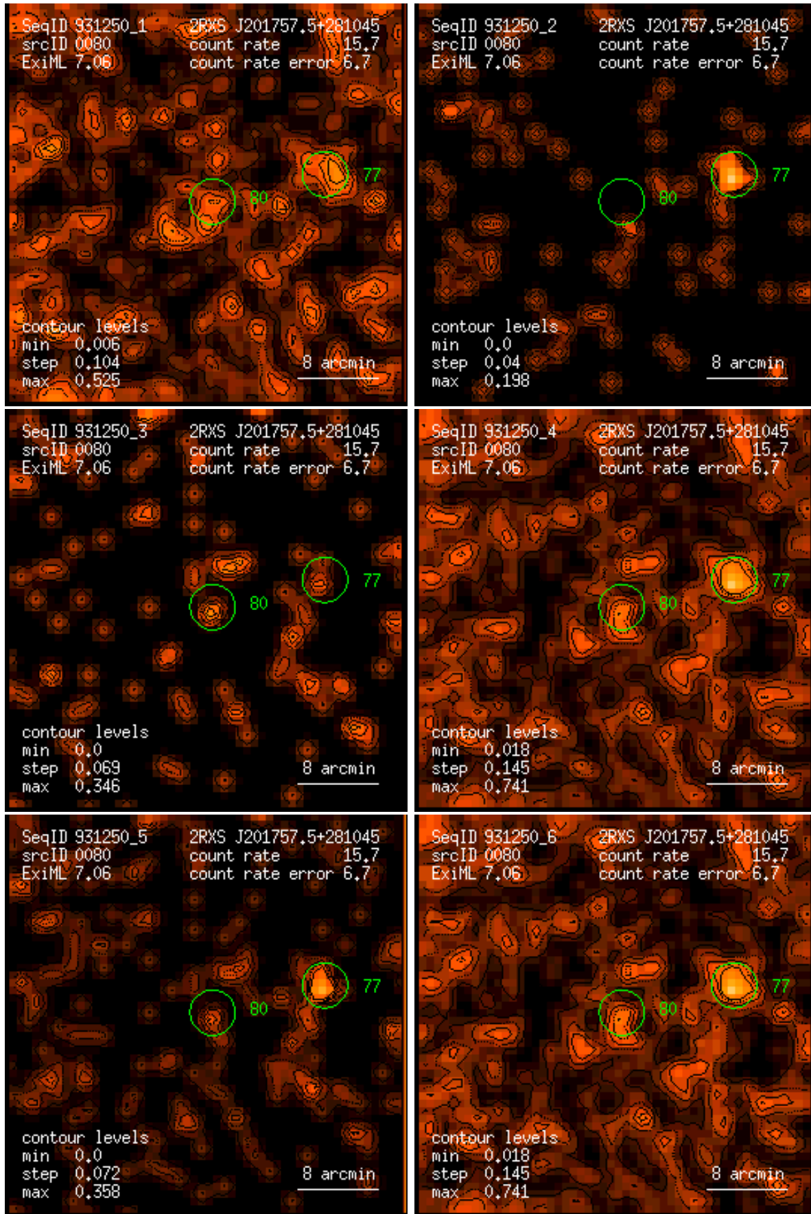
Figure 80: RASS 931250: detection 0080: band rate images, Gaussian filter: (1) PSPC channels 11 – 41, (2) 52 – 90, (3) 91 – 201, (4) 11 – 235, (5) 52 – 201, (6) 11 – 201. Broad band rates in counts/ks. Band rate contour levels in counts/ks/arcmin 2 .
