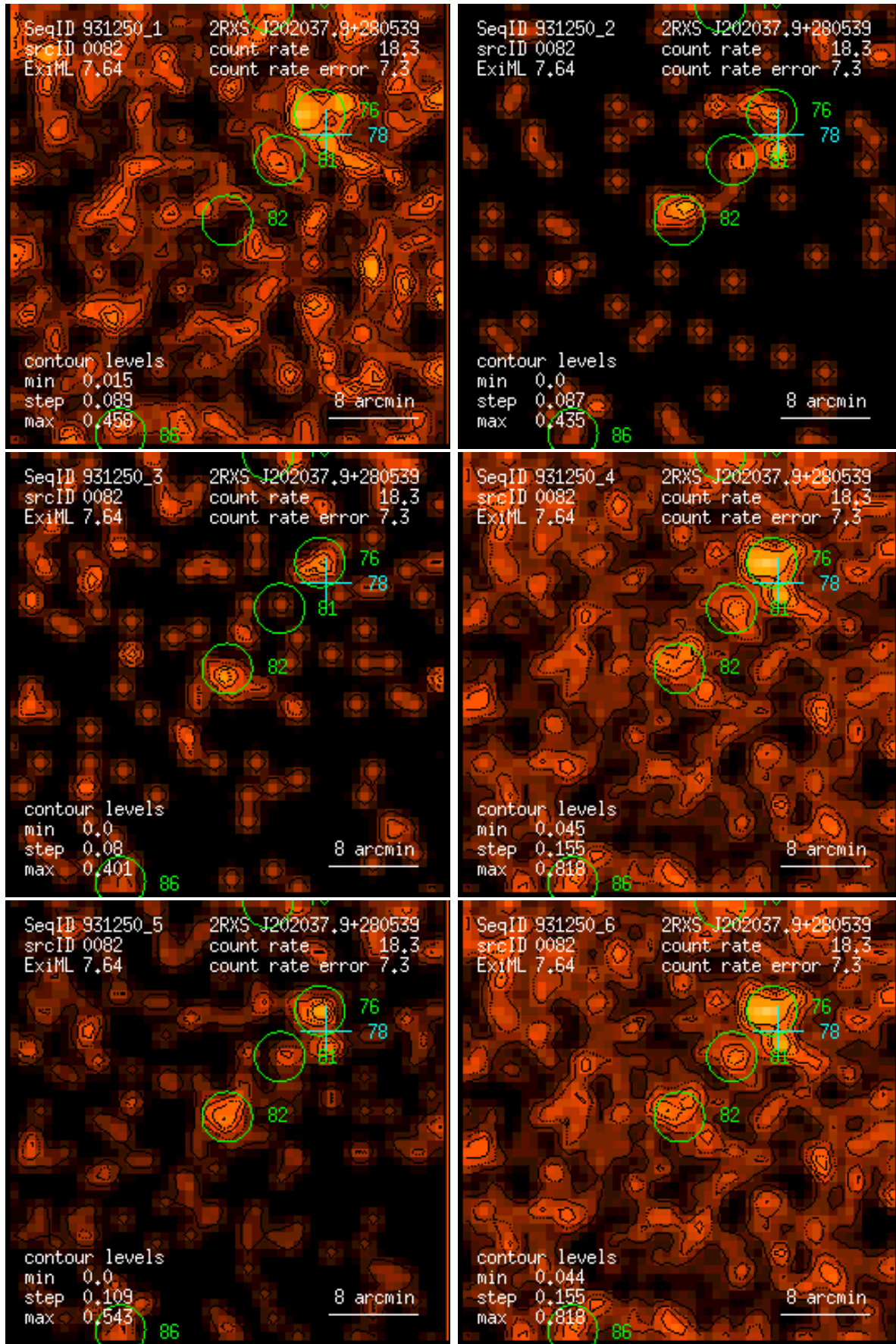
Figure 82: RASS 931250: detection 0082: band rate images, Gaussian filter: (1) PSPC channels 11 – 41, (2) 52 – 90, (3) 91 – 201, (4) 11 – 235, (5) 52 – 201, (6) 11 – 201. Broad band rates in counts/ks. Band rate contour levels in counts/ks/arcmin 2 .
