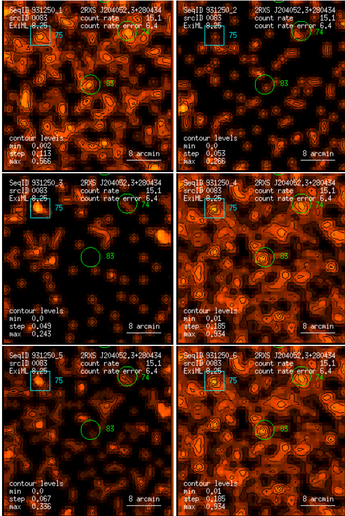
Figure 83: RASS 931250: detection 0083: band rate images, Gaussian filter: (1) PSPC channels 11 – 41, (2) 52 – 90, (3) 91 – 201, (4) 11 – 235, (5) 52 – 201, (6) 11 – 201. Broad band rates in counts/ks. Band rate contour levels in counts/ks/arcmin 2 .
