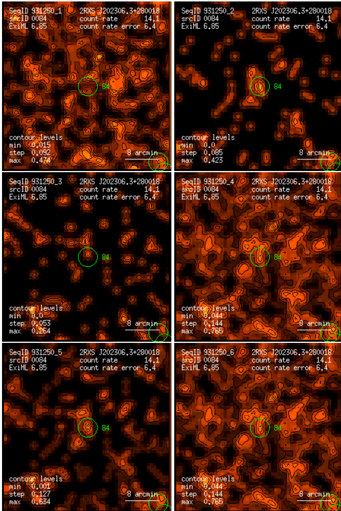
Figure 84: RASS 931250: detection 0084: band rate images, Gaussian filter: (1) PSPC channels 11 – 41, (2) 52 – 90, (3) 91 – 201, (4) 11 – 235, (5) 52 – 201, (6) 11 – 201. Broad band rates in counts/ks. Band rate contour levels in counts/ks/arcmin 2 .
