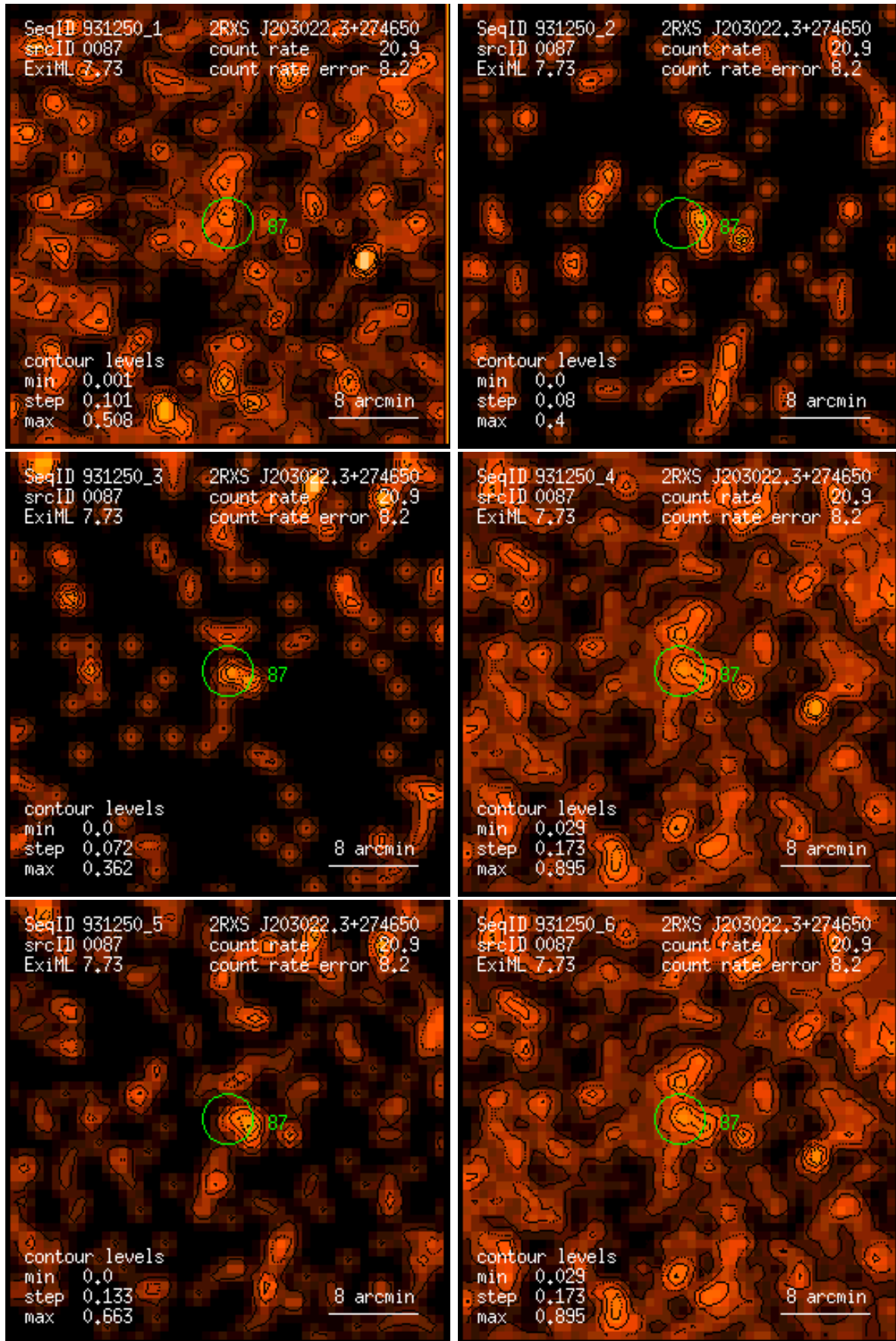
Figure 87: RASS 931250: detection 0087: band rate images, Gaussian filter: (1) PSPC channels 11 – 41, (2) 52 – 90, (3) 91 – 201, (4) 11 – 235, (5) 52 – 201, (6) 11 – 201. Broad band rates in counts/ks. Band rate contour levels in counts/ks/arcmin 2 .
