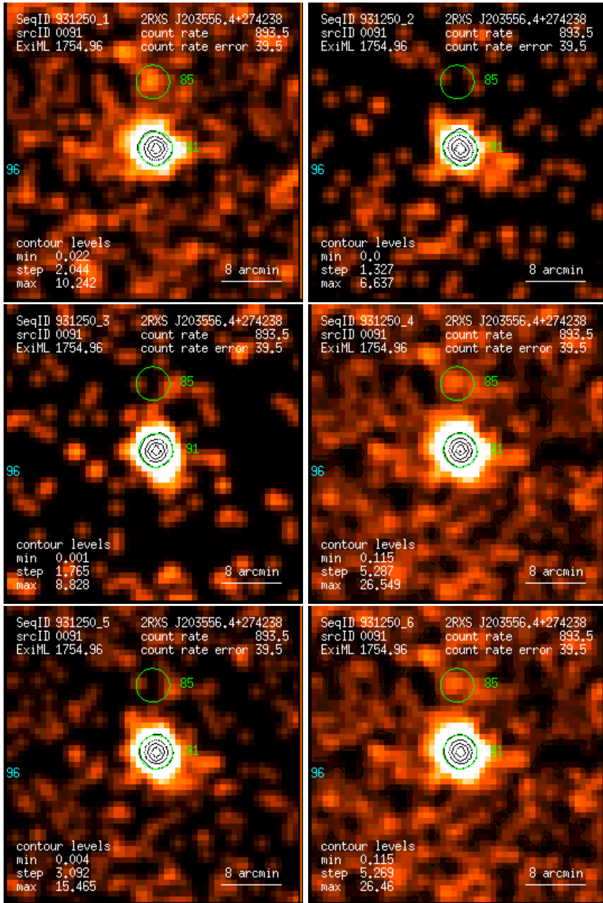
Figure 91: RASS 931250: detection 0091: band rate images, Gaussian filter: (1) PSPC channels 11 – 41, (2) 52 – 90, (3) 91 – 201, (4) 11 – 235, (5) 52 – 201, (6) 11 – 201. Broad band rates in counts/ks. Band rate contour levels in counts/ks/arcmin 2 .
