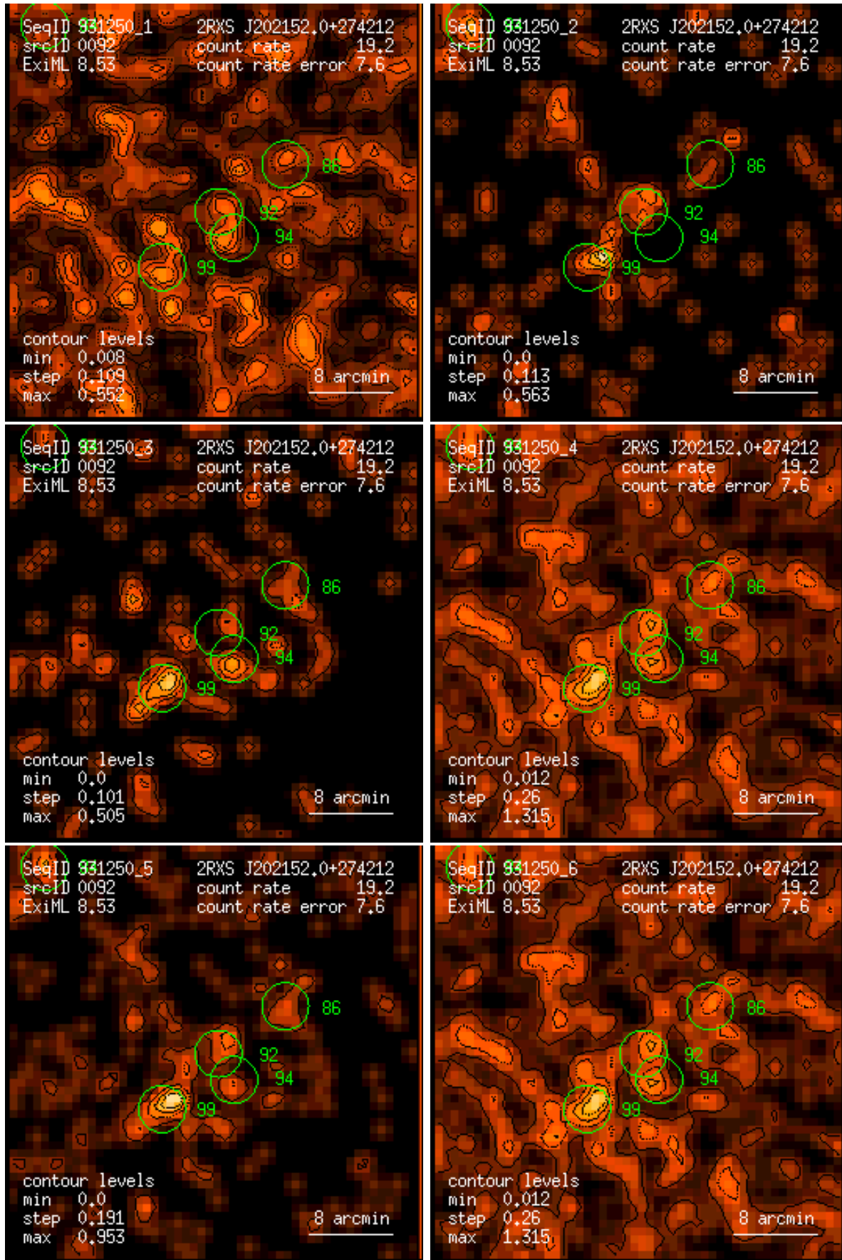
Figure 92: RASS 931250: detection 0092: band rate images, Gaussian filter: (1) PSPC channels 11 – 41, (2) 52 – 90, (3) 91 – 201, (4) 11 – 235, (5) 52 – 201, (6) 11 – 201. Broad band rates in counts/ks. Band rate contour levels in counts/ks/arcmin 2 .
