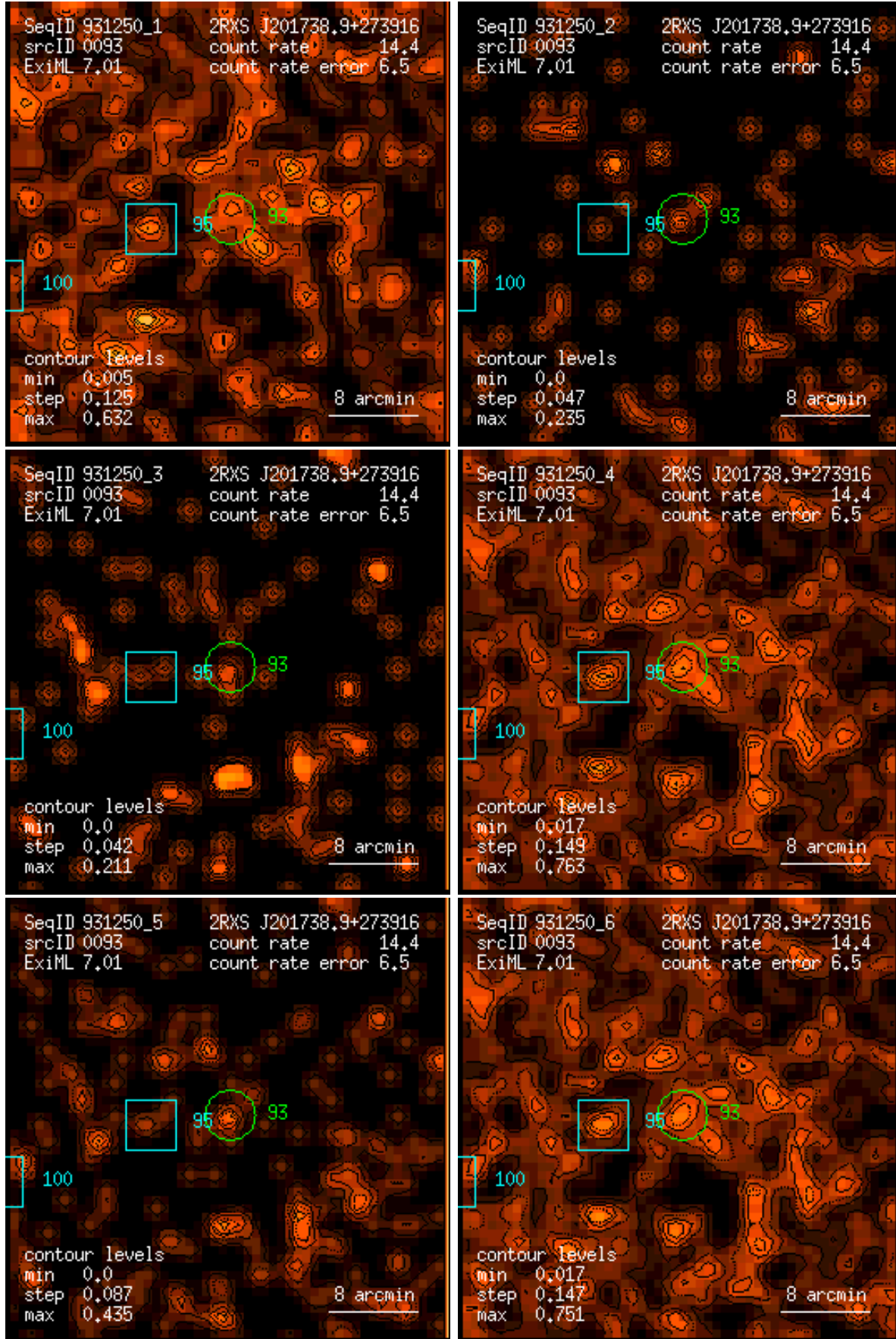
Figure 93: RASS 931250: detection 0093: band rate images, Gaussian filter: (1) PSPC channels 11 – 41, (2) 52 – 90, (3) 91 – 201, (4) 11 – 235, (5) 52 – 201, (6) 11 – 201. Broad band rates in counts/ks. Band rate contour levels in counts/ks/arcmin 2 .
