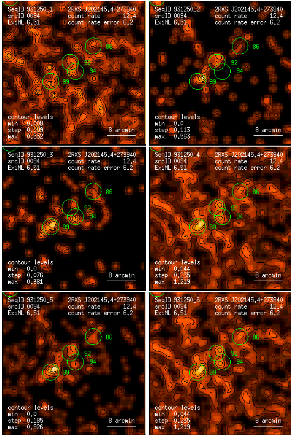
Figure 94: RASS 931250: detection 0094: band rate images, Gaussian filter: (1) PSPC channels 11 – 41, (2) 52 – 90, (3) 91 – 201, (4) 11 – 235, (5) 52 – 201, (6) 11 – 201. Broad band rates in counts/ks. Band rate contour levels in counts/ks/arcmin 2 .
