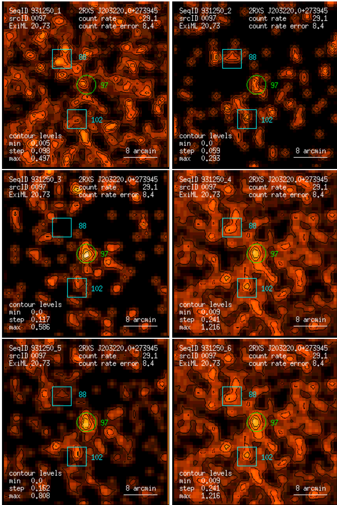
Figure 97: RASS 931250: detection 0097: band rate images, Gaussian filter: (1) PSPC channels 11 – 41, (2) 52 – 90, (3) 91 – 201, (4) 11 – 235, (5) 52 – 201, (6) 11 – 201. Broad band rates in counts/ks. Band rate contour levels in counts/ks/arcmin 2 .
