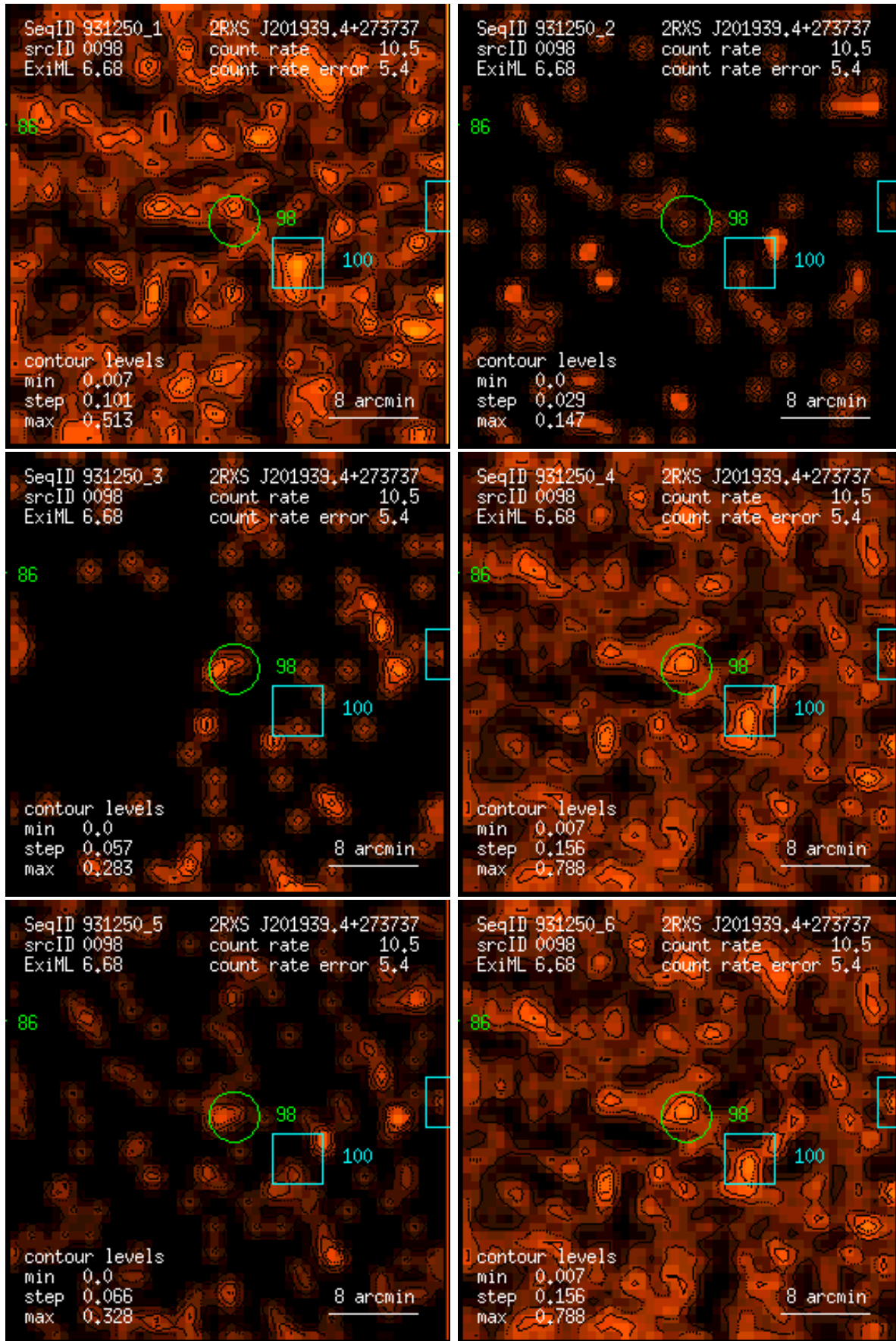
Figure 98: RASS 931250: detection 0098: band rate images, Gaussian filter: (1) PSPC channels 11 – 41, (2) 52 – 90, (3) 91 – 201, (4) 11 – 235, (5) 52 – 201, (6) 11 – 201. Broad band rates in counts/ks. Band rate contour levels in counts/ks/arcmin 2 .
