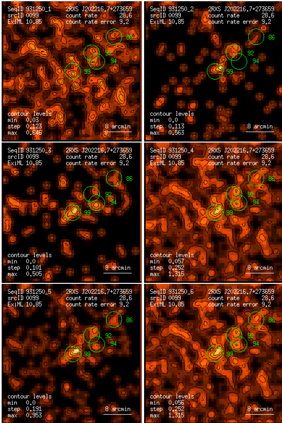
Figure 99: RASS 931250: detection 0099: band rate images, Gaussian filter: (1) PSPC channels 11 – 41, (2) 52 – 90, (3) 91 – 201, (4) 11 – 235, (5) 52 – 201, (6) 11 – 201. Broad band rates in counts/ks. Band rate contour levels in counts/ks/arcmin 2 .
