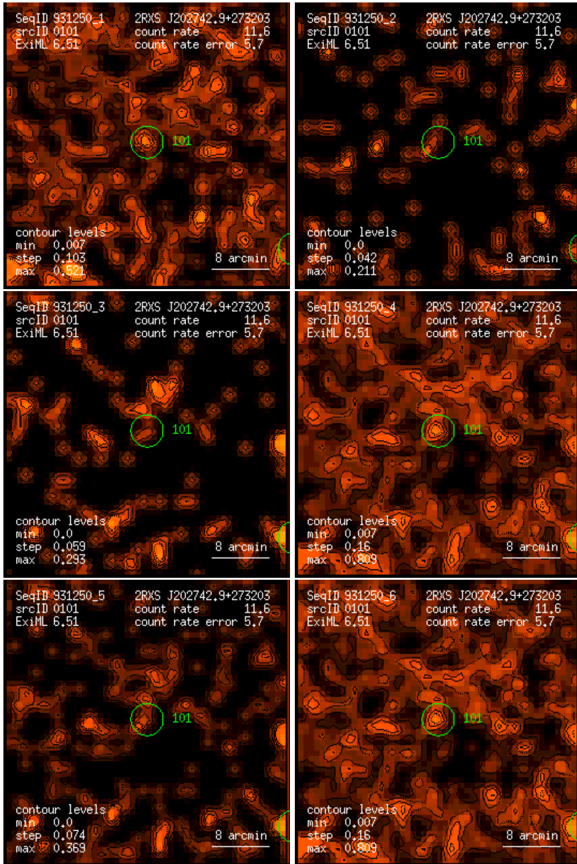
Figure 101: RASS 931250: detection 0101: band rate images, Gaussian filter: (1) PSPC channels 11 – 41, (2) 52 – 90, (3) 91 – 201, (4) 11 – 235, (5) 52 – 201, (6) 11 – 201. Broad band rates in counts/ks. Band rate contour levels in counts/ks/arcmin 2 .
