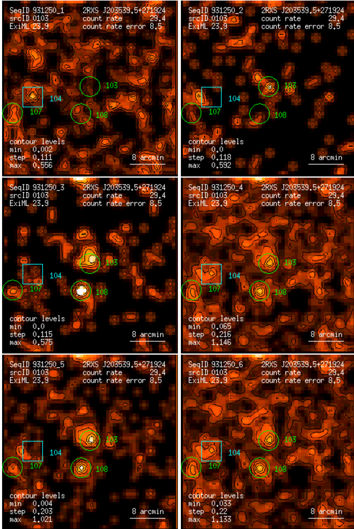
Figure 103: RASS 931250: detection 0103: band rate images, Gaussian filter: (1) PSPC channels 11 – 41, (2) 52 – 90, (3) 91 – 201, (4) 11 – 235, (5) 52 – 201, (6) 11 – 201. Broad band rates in counts/ks. Band rate contour levels in counts/ks/arcmin 2 .
