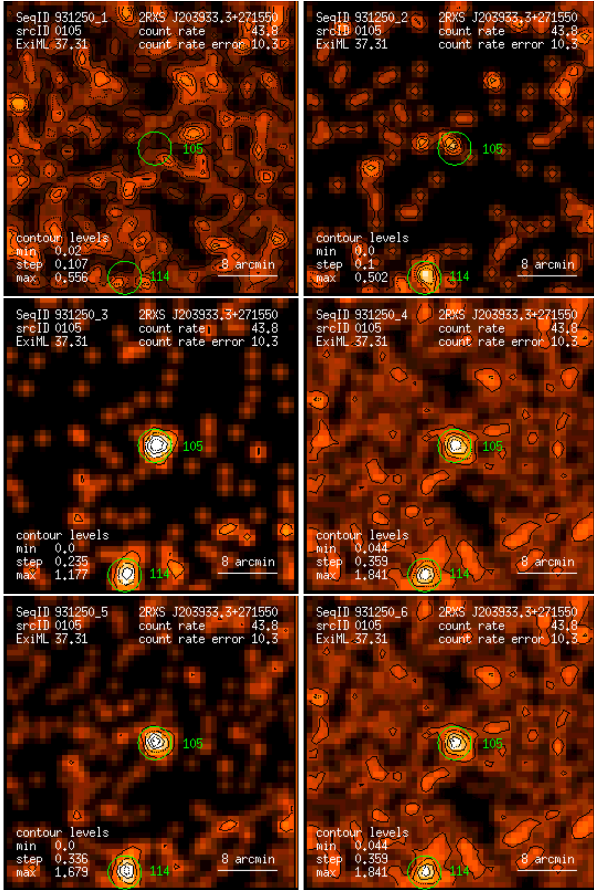
Figure 105: RASS 931250: detection 0105: band rate images, Gaussian filter: (1) PSPC channels 11 – 41, (2) 52 – 90, (3) 91 – 201, (4) 11 – 235, (5) 52 – 201, (6) 11 – 201. Broad band rates in counts/ks. Band rate contour levels in counts/ks/arcmin 2 .
