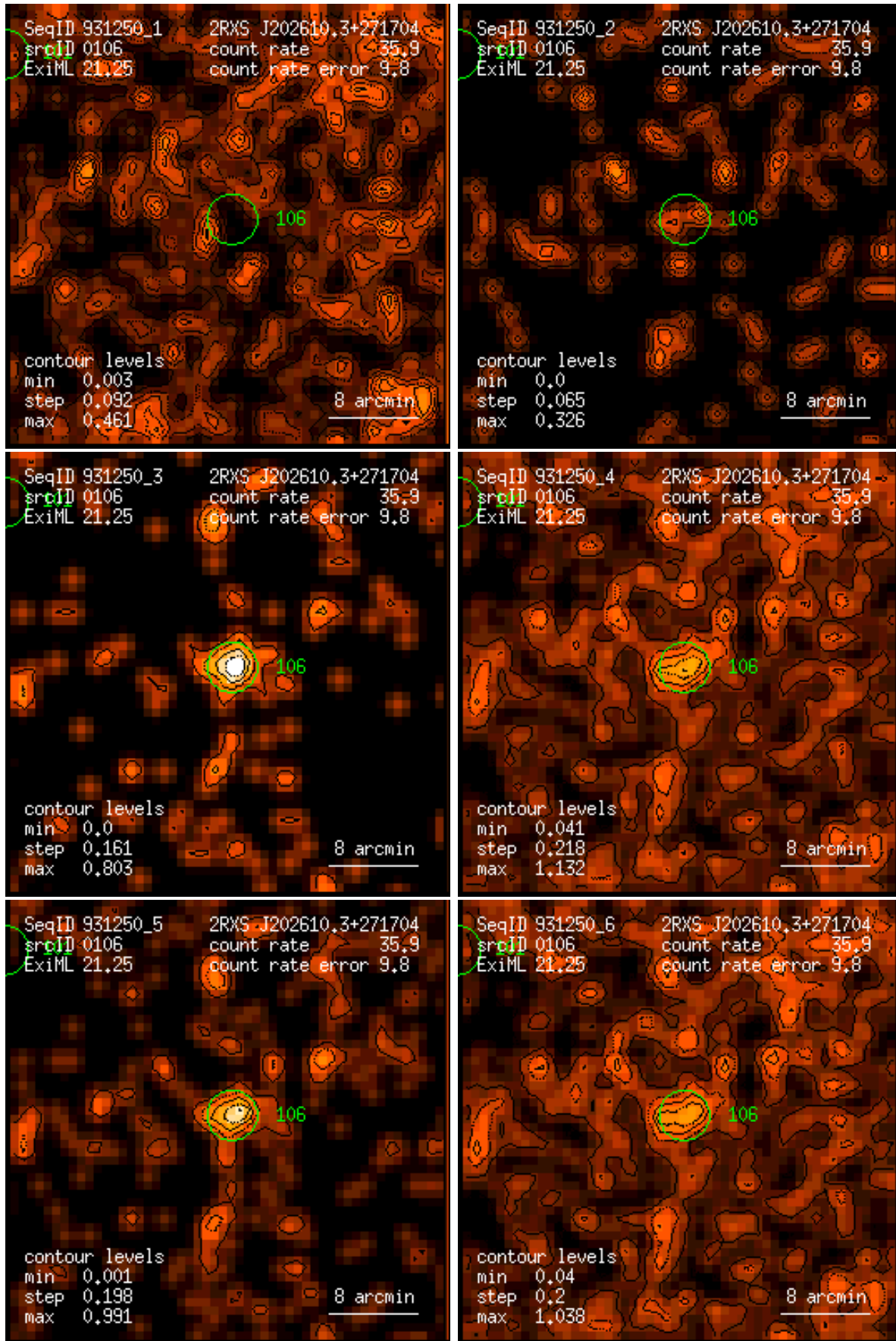
Figure 106: RASS 931250: detection 0106: band rate images, Gaussian filter: (1) PSPC channels 11 – 41, (2) 52 – 90, (3) 91 – 201, (4) 11 – 235, (5) 52 – 201, (6) 11 – 201. Broad band rates in counts/ks. Band rate contour levels in counts/ks/arcmin 2 .
