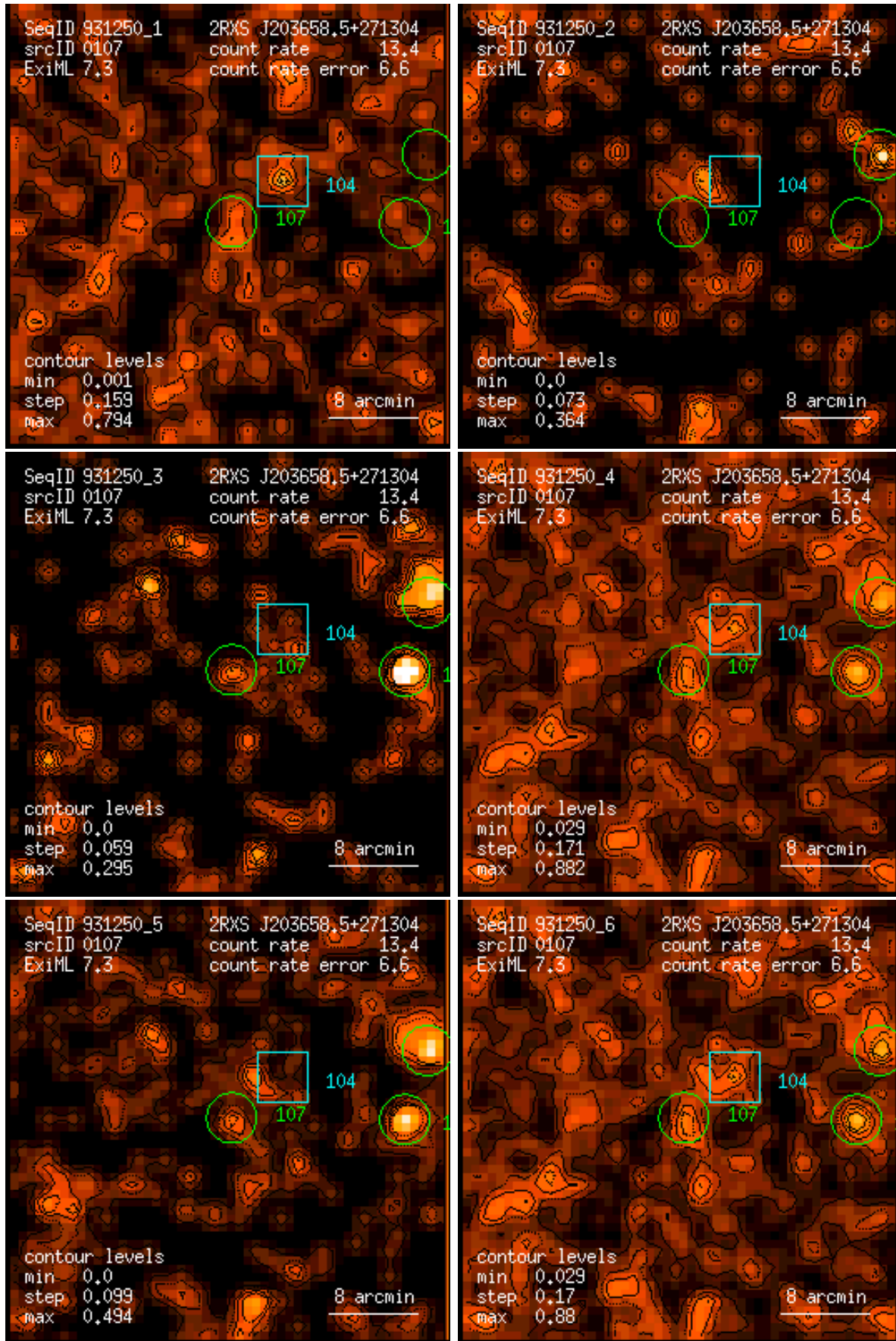
Figure 107: RASS 931250: detection 0107: band rate images, Gaussian filter: (1) PSPC channels 11 – 41, (2) 52 – 90, (3) 91 – 201, (4) 11 – 235, (5) 52 – 201, (6) 11 – 201. Broad band rates in counts/ks. Band rate contour levels in counts/ks/arcmin 2 .
