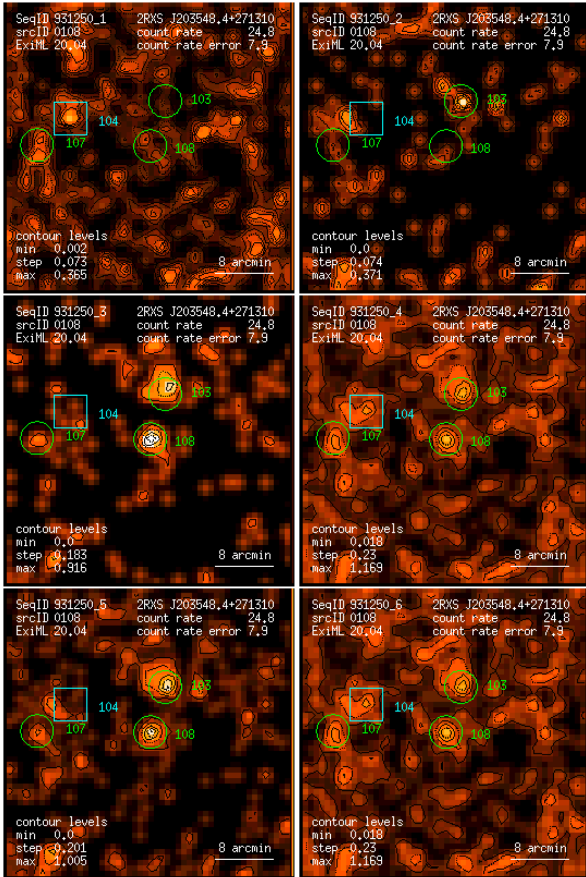
Figure 108: RASS 931250: detection 0108: band rate images, Gaussian filter: (1) PSPC channels 11 – 41, (2) 52 – 90, (3) 91 – 201, (4) 11 – 235, (5) 52 – 201, (6) 11 – 201. Broad band rates in counts/ks. Band rate contour levels in counts/ks/arcmin 2 .
