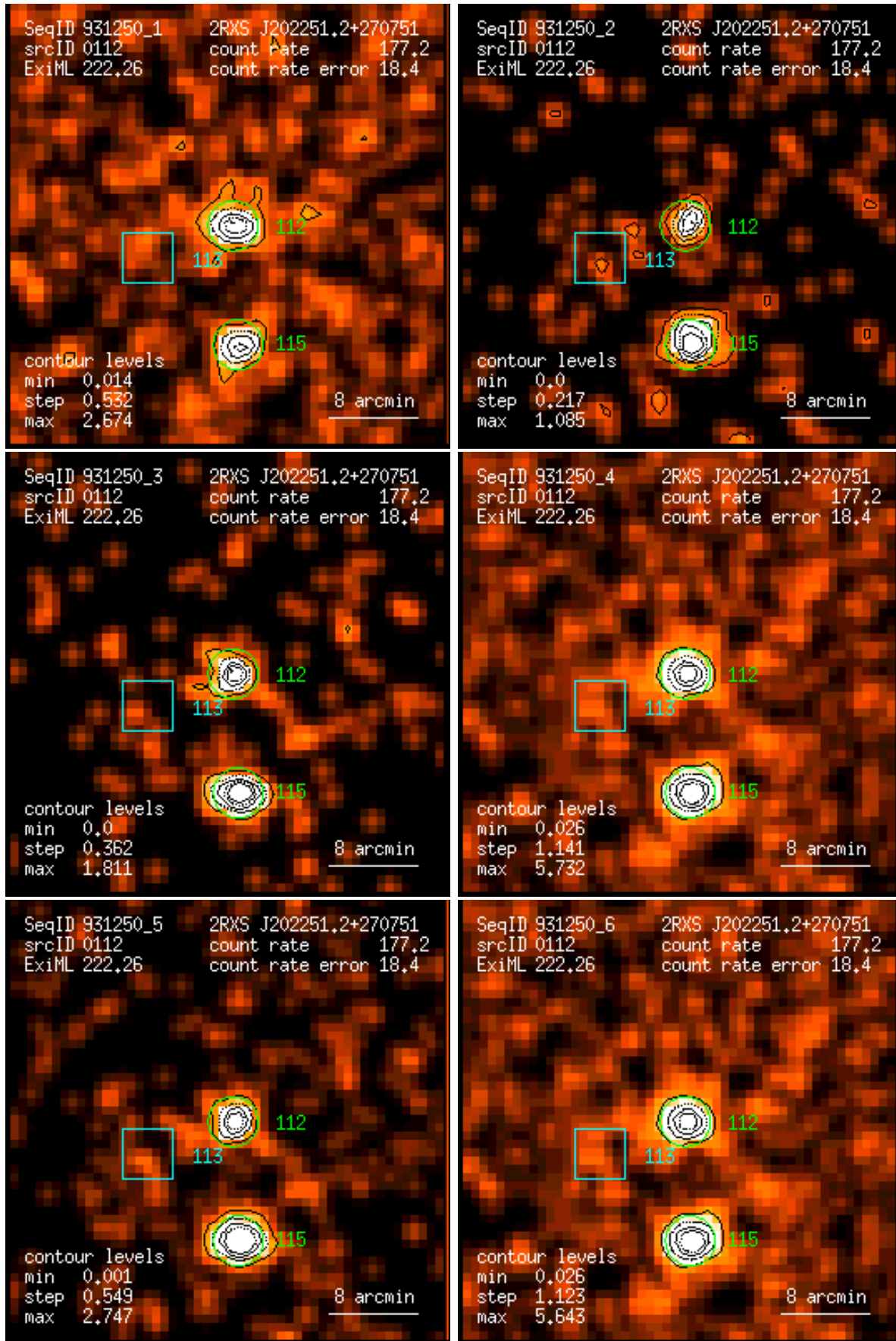
Figure 112: RASS 931250: detection 0112: band rate images, Gaussian filter: (1) PSPC channels 11 – 41, (2) 52 – 90, (3) 91 – 201, (4) 11 – 235, (5) 52 – 201, (6) 11 – 201. Broad band rates in counts/ks. Band rate contour levels in counts/ks/arcmin 2 .
