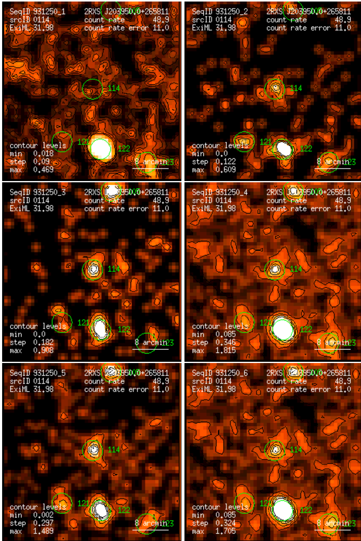
Figure 114: RASS 931250: detection 0114: band rate images, Gaussian filter: (1) PSPC channels 11 – 41, (2) 52 – 90, (3) 91 – 201, (4) 11 – 235, (5) 52 – 201, (6) 11 – 201. Broad band rates in counts/ks. Band rate contour levels in counts/ks/arcmin 2 .
