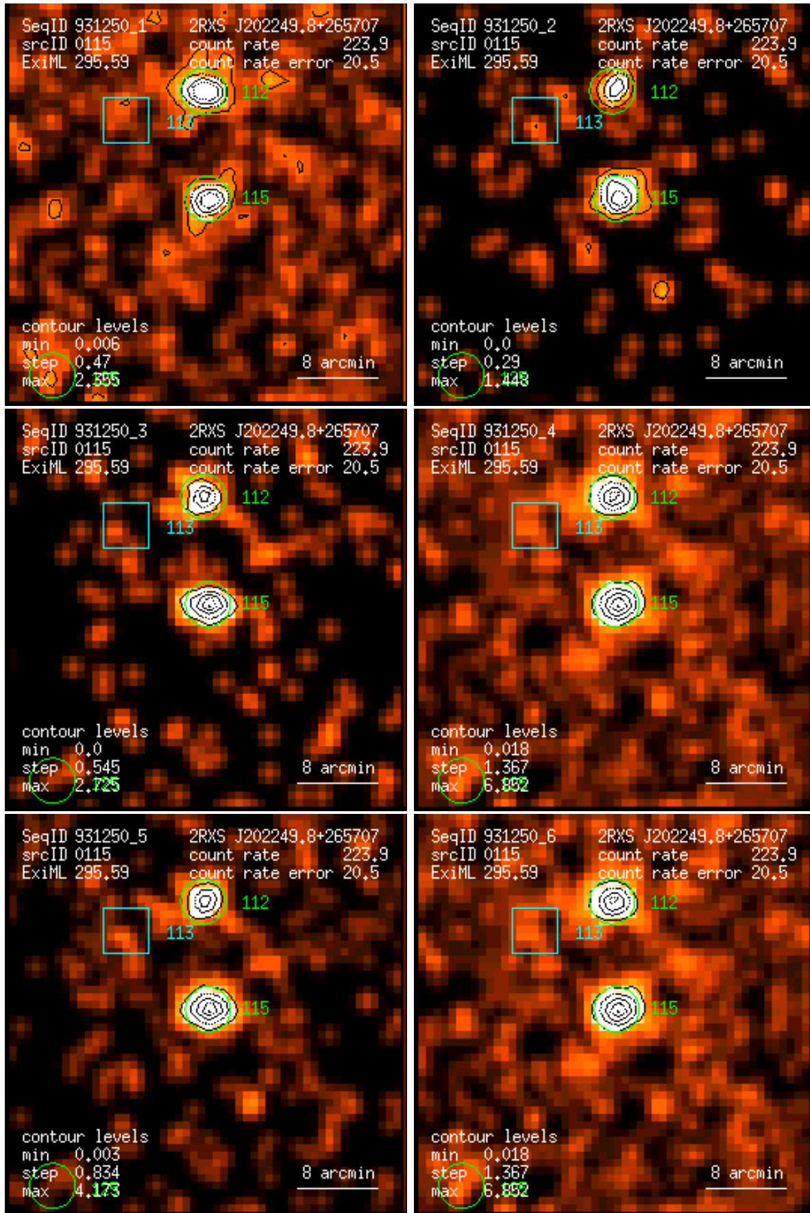
Figure 115: RASS 931250: detection 0115: band rate images, Gaussian filter: (1) PSPC channels 11 – 41, (2) 52 – 90, (3) 91 – 201, (4) 11 – 235, (5) 52 – 201, (6) 11 – 201. Broad band rates in counts/ks. Band rate contour levels in counts/ks/arcmin 2 .
