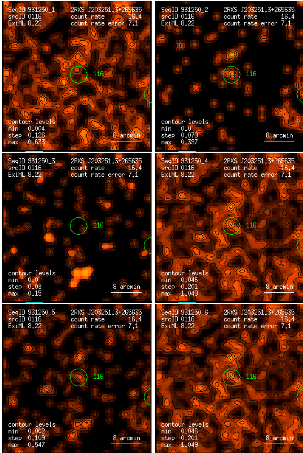
Figure 116: RASS 931250: detection 0116: band rate images, Gaussian filter: (1) PSPC channels 11 – 41, (2) 52 – 90, (3) 91 – 201, (4) 11 – 235, (5) 52 – 201, (6) 11 – 201. Broad band rates in counts/ks. Band rate contour levels in counts/ks/arcmin 2 .
