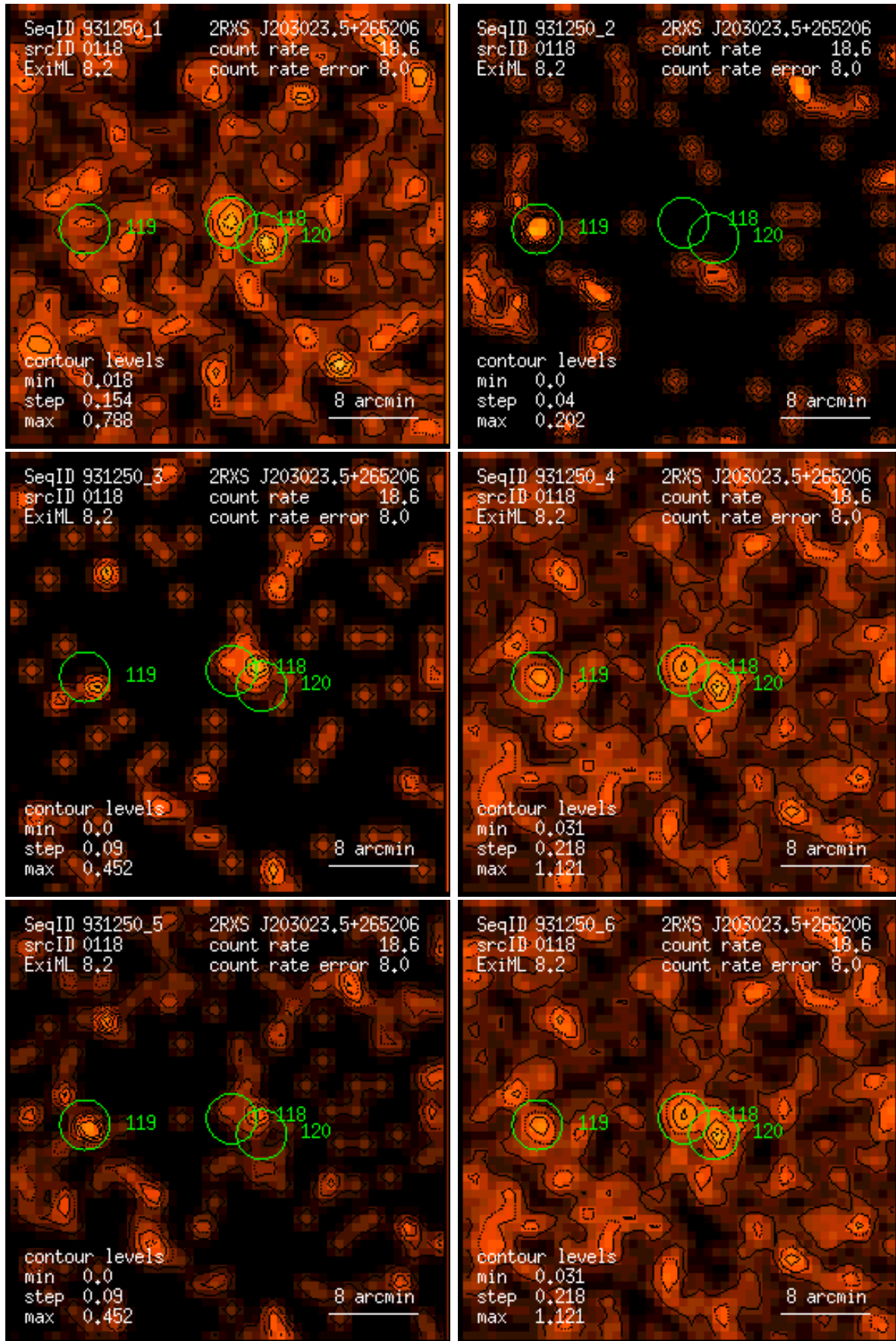
Figure 118: RASS 931250: detection 0118: band rate images, Gaussian filter: (1) PSPC channels 11 – 41, (2) 52 – 90, (3) 91 – 201, (4) 11 – 235, (5) 52 – 201, (6) 11 – 201. Broad band rates in counts/ks. Band rate contour levels in counts/ks/arcmin 2 .
