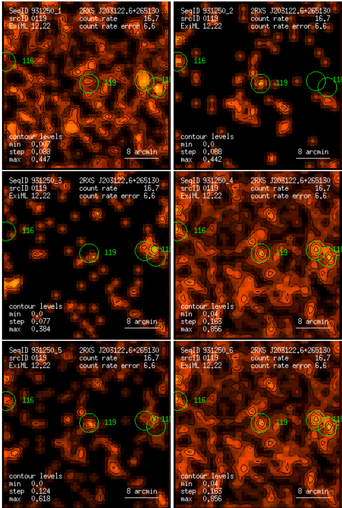
Figure 119: RASS 931250: detection 0119: band rate images, Gaussian filter: (1) PSPC channels 11 – 41, (2) 52 – 90, (3) 91 – 201, (4) 11 – 235, (5) 52 – 201, (6) 11 – 201. Broad band rates in counts/ks. Band rate contour levels in counts/ks/arcmin 2 .
