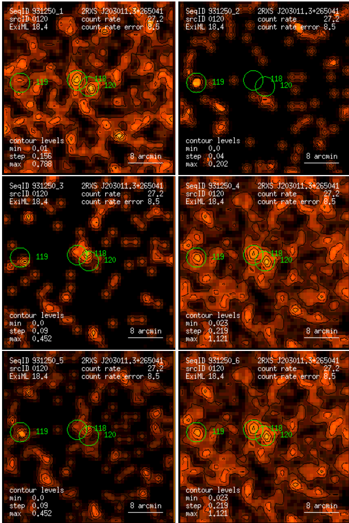
Figure 120: RASS 931250: detection 0120: band rate images, Gaussian filter: (1) PSPC channels 11 – 41, (2) 52 – 90, (3) 91 – 201, (4) 11 – 235, (5) 52 – 201, (6) 11 – 201. Broad band rates in counts/ks. Band rate contour levels in counts/ks/arcmin 2 .
