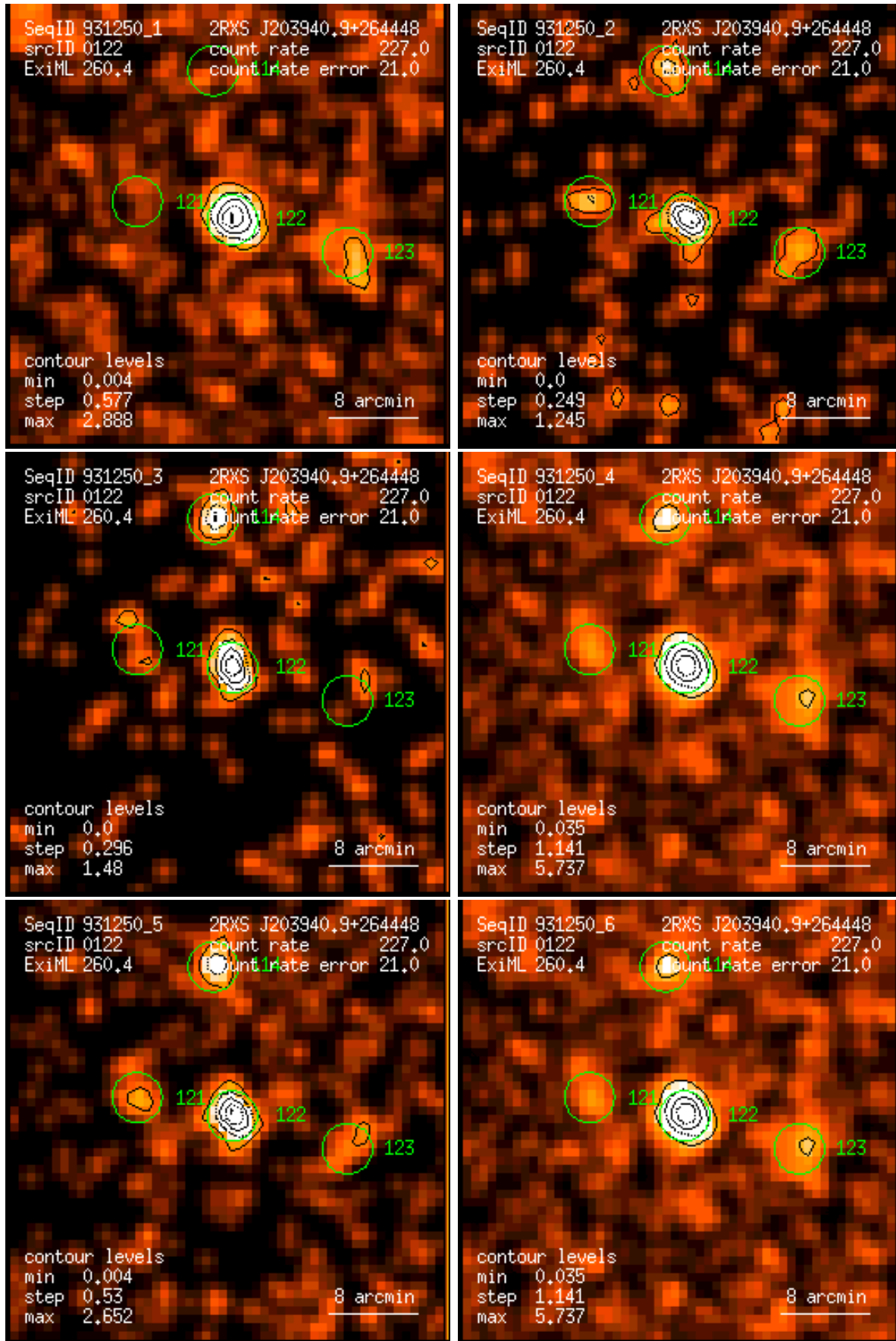
Figure 122: RASS 931250: detection 0122: band rate images, Gaussian filter: (1) PSPC channels 11 – 41, (2) 52 – 90, (3) 91 – 201, (4) 11 – 235, (5) 52 – 201, (6) 11 – 201. Broad band rates in counts/ks. Band rate contour levels in counts/ks/arcmin 2 .
