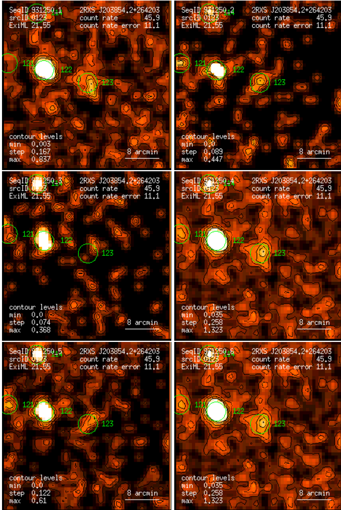
Figure 123: RASS 931250: detection 0123: band rate images, Gaussian filter: (1) PSPC channels 11 – 41, (2) 52 – 90, (3) 91 – 201, (4) 11 – 235, (5) 52 – 201, (6) 11 – 201. Broad band rates in counts/ks. Band rate contour levels in counts/ks/arcmin 2 .
