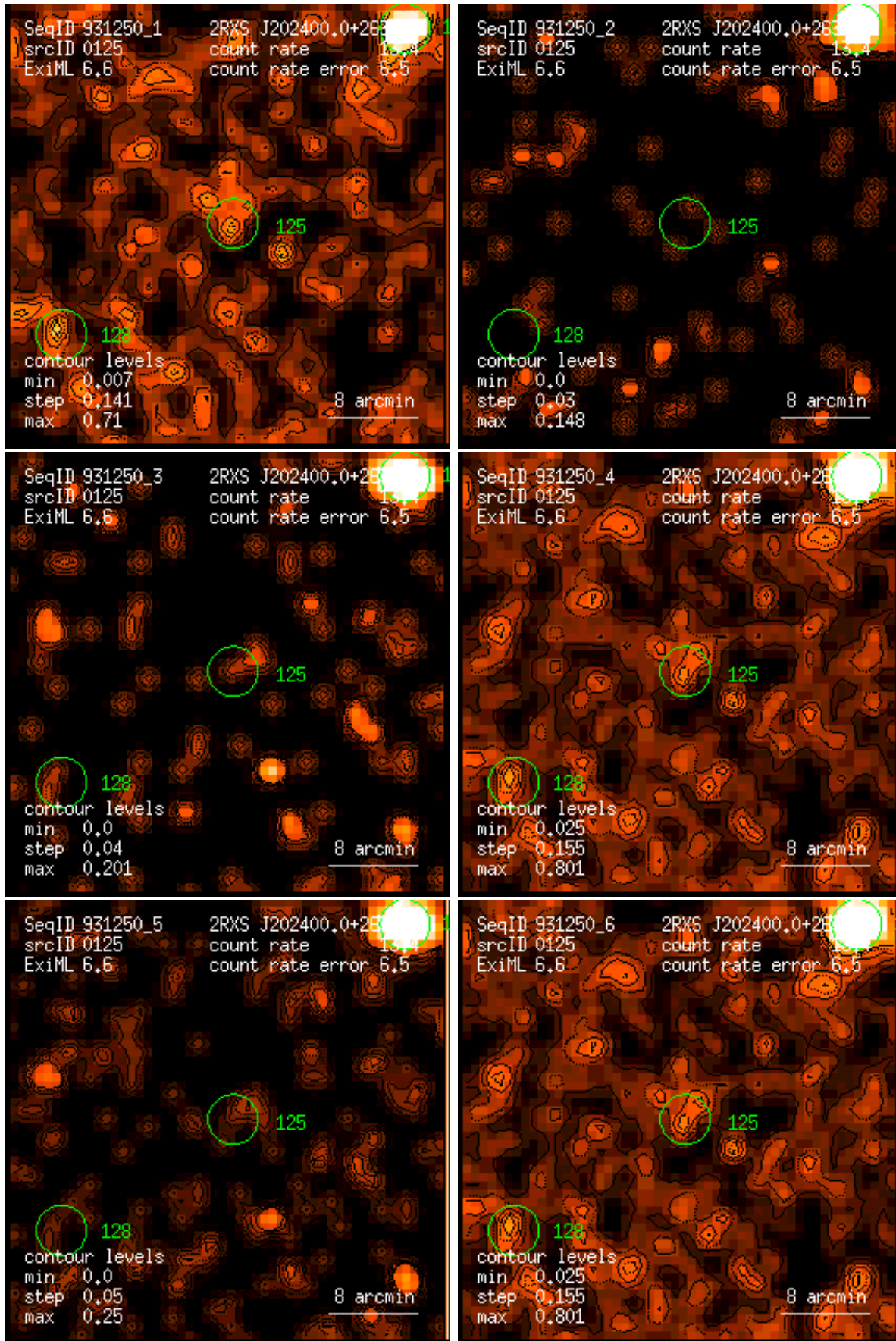
Figure 125: RASS 931250: detection 0125: band rate images, Gaussian filter: (1) PSPC channels 11 – 41, (2) 52 – 90, (3) 91 – 201, (4) 11 – 235, (5) 52 – 201, (6) 11 – 201. Broad band rates in counts/ks. Band rate contour levels in counts/ks/arcmin 2 .
