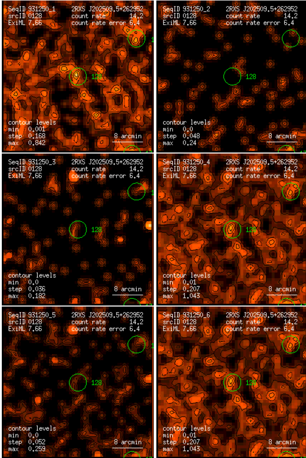
Figure 128: RASS 931250: detection 0128: band rate images, Gaussian filter: (1) PSPC channels 11 – 41, (2) 52 – 90, (3) 91 – 201, (4) 11 – 235, (5) 52 – 201, (6) 11 – 201. Broad band rates in counts/ks. Band rate contour levels in counts/ks/arcmin 2 .
