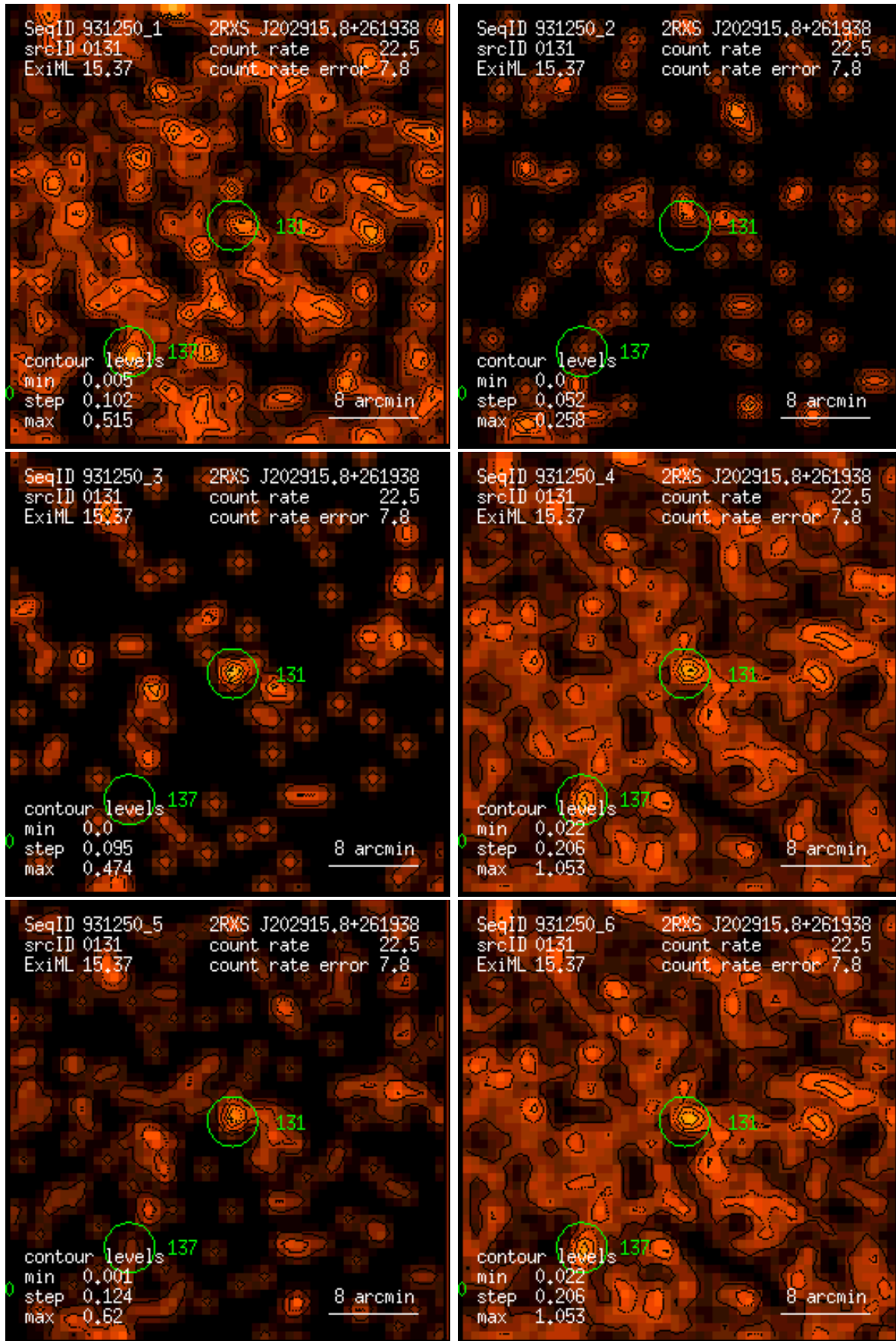
Figure 131: RASS 931250: detection 0131: band rate images, Gaussian filter: (1) PSPC channels 11 – 41, (2) 52 – 90, (3) 91 – 201, (4) 11 – 235, (5) 52 – 201, (6) 11 – 201. Broad band rates in counts/ks. Band rate contour levels in counts/ks/arcmin 2 .
