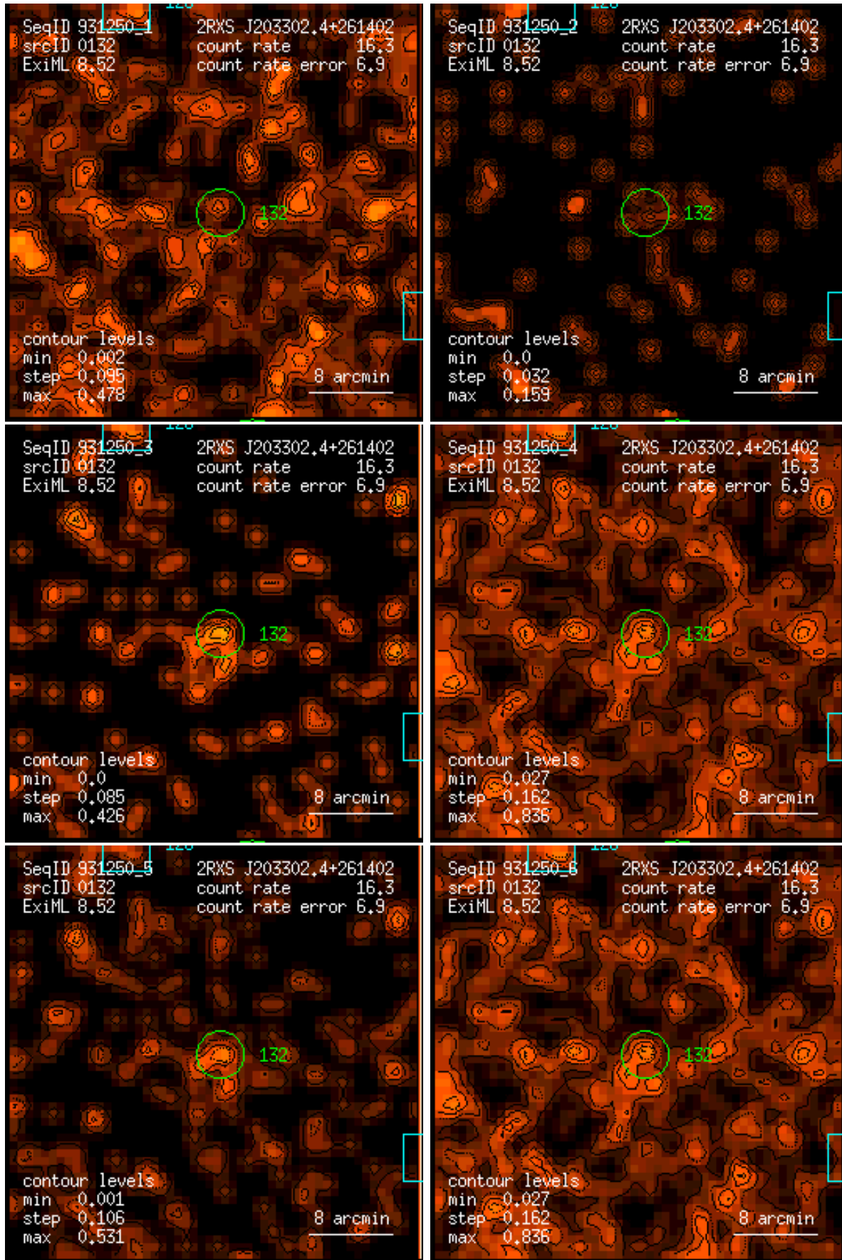
Figure 132: RASS 931250: detection 0132: band rate images, Gaussian filter: (1) PSPC channels 11 – 41, (2) 52 – 90, (3) 91 – 201, (4) 11 – 235, (5) 52 – 201, (6) 11 – 201. Broad band rates in counts/ks. Band rate contour levels in counts/ks/arcmin 2 .
