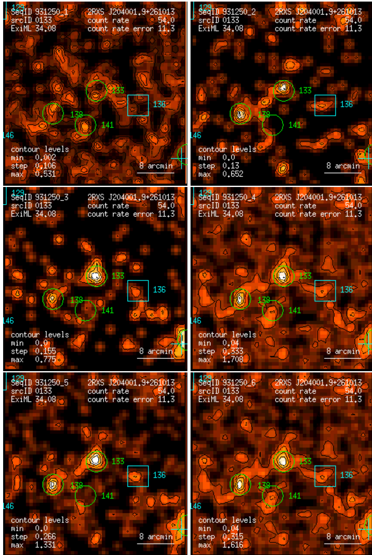
Figure 133: RASS 931250: detection 0133: band rate images, Gaussian filter: (1) PSPC channels 11 – 41, (2) 52 – 90, (3) 91 – 201, (4) 11 – 235, (5) 52 – 201, (6) 11 – 201. Broad band rates in counts/ks. Band rate contour levels in counts/ks/arcmin 2 .
