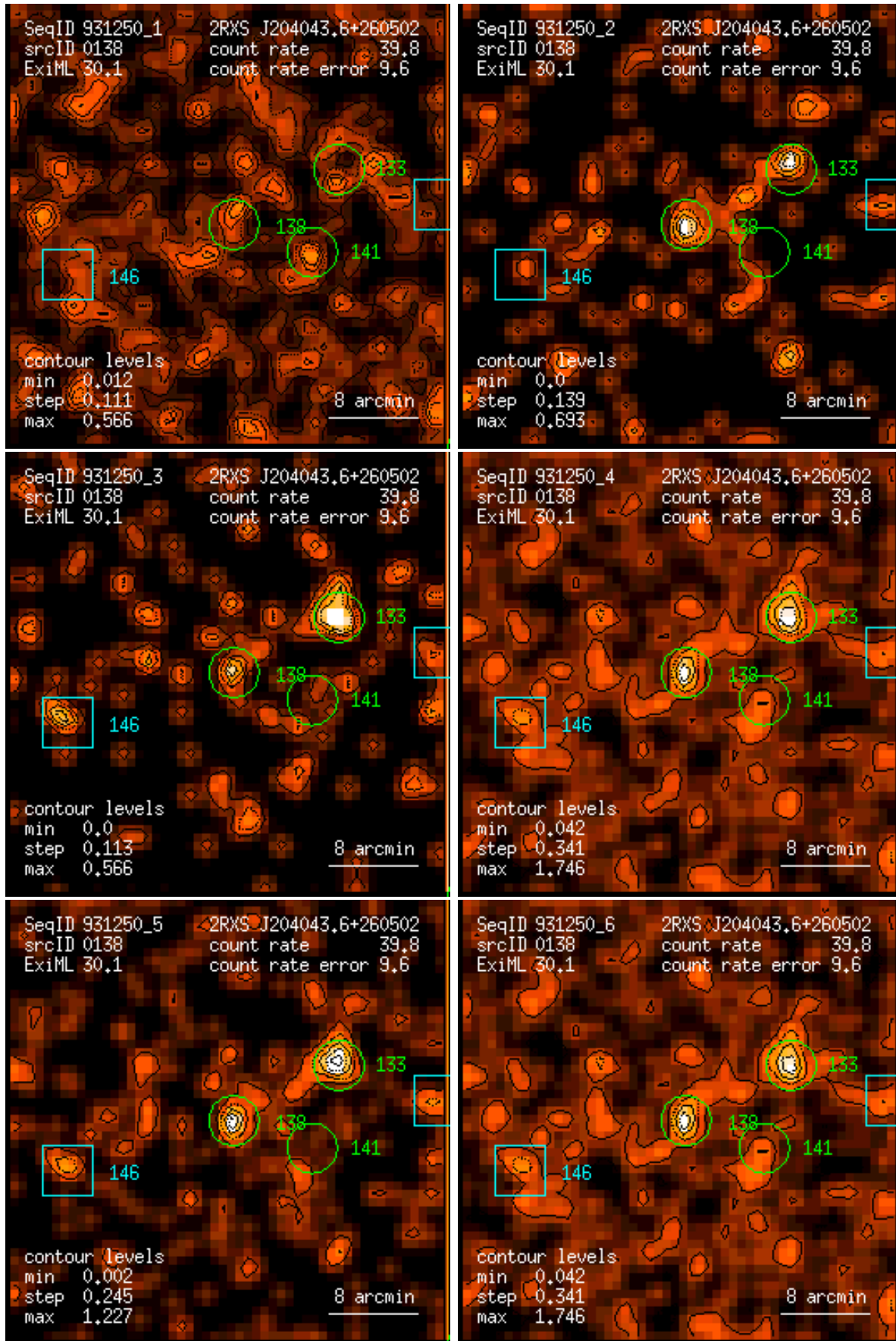
Figure 138: RASS 931250: detection 0138: band rate images, Gaussian filter: (1) PSPC channels 11 – 41, (2) 52 – 90, (3) 91 – 201, (4) 11 – 235, (5) 52 – 201, (6) 11 – 201. Broad band rates in counts/ks. Band rate contour levels in counts/ks/arcmin 2 .
