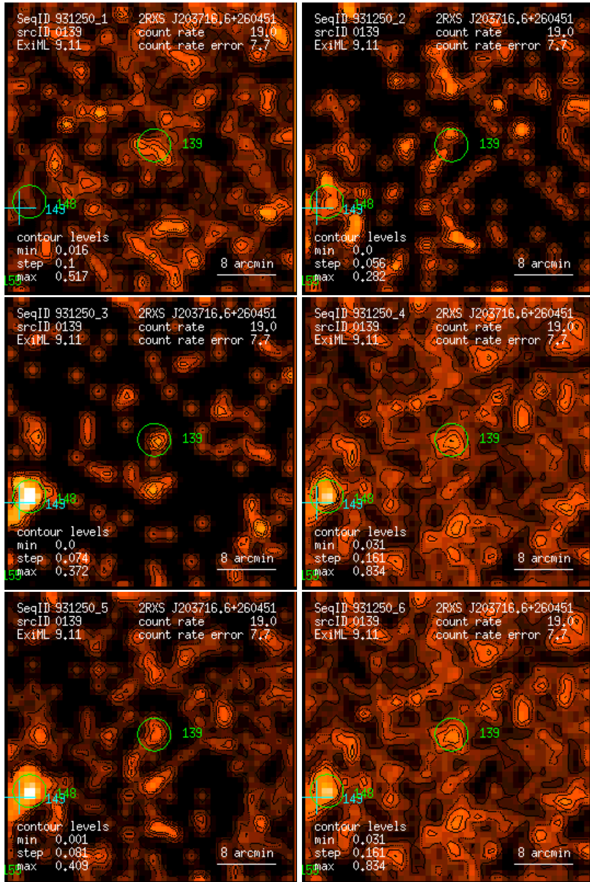
Figure 139: RASS 931250: detection 0139: band rate images, Gaussian filter: (1) PSPC channels 11 – 41, (2) 52 – 90, (3) 91 – 201, (4) 11 – 235, (5) 52 – 201, (6) 11 – 201. Broad band rates in counts/ks. Band rate contour levels in counts/ks/arcmin 2 .
