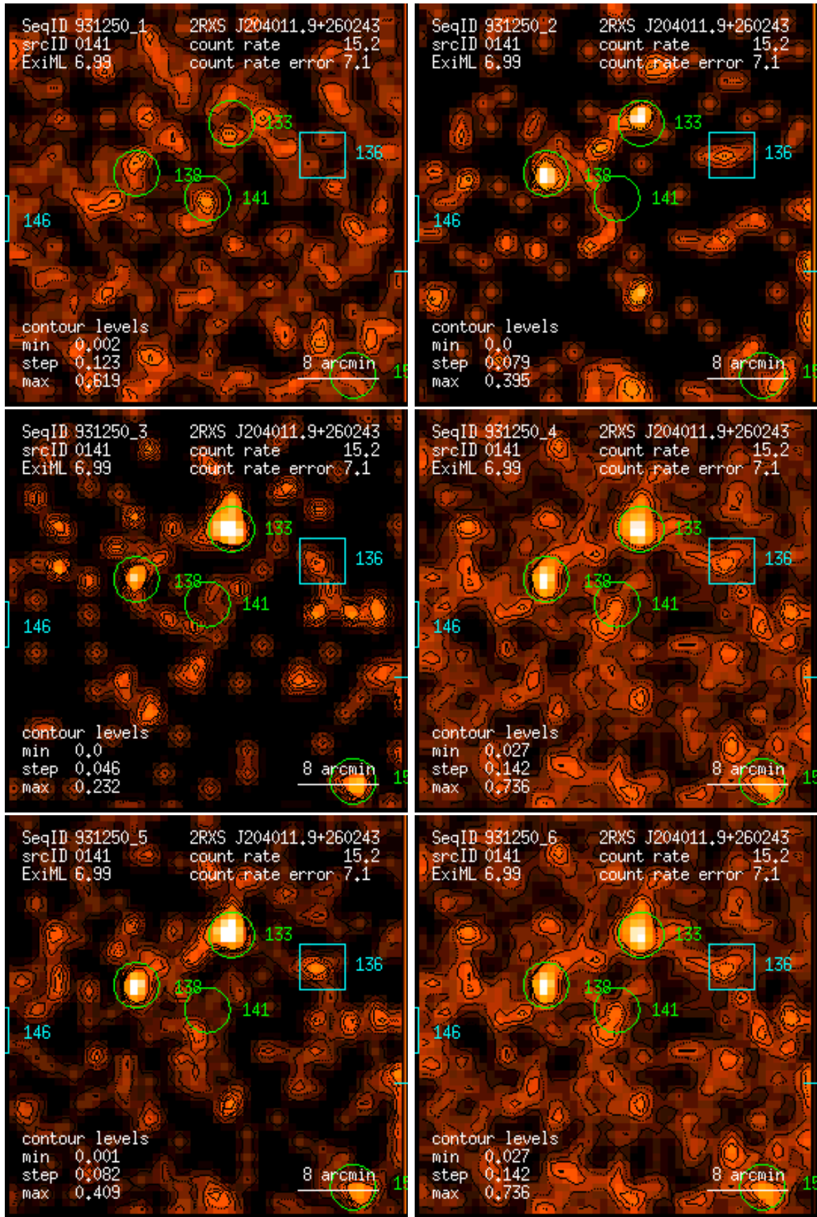
Figure 141: RASS 931250: detection 0141: band rate images, Gaussian filter: (1) PSPC channels 11 – 41, (2) 52 – 90, (3) 91 – 201, (4) 11 – 235, (5) 52 – 201, (6) 11 – 201. Broad band rates in counts/ks. Band rate contour levels in counts/ks/arcmin 2 .
