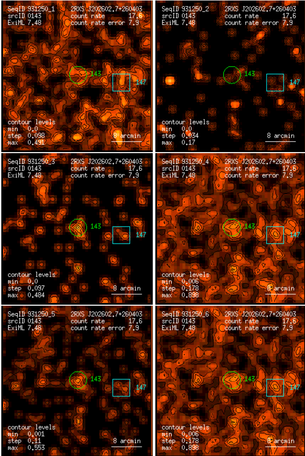
Figure 143: RASS 931250: detection 0143: band rate images, Gaussian filter: (1) PSPC channels 11 – 41, (2) 52 – 90, (3) 91 – 201, (4) 11 – 235, (5) 52 – 201, (6) 11 – 201. Broad band rates in counts/ks. Band rate contour levels in counts/ks/arcmin 2 .
