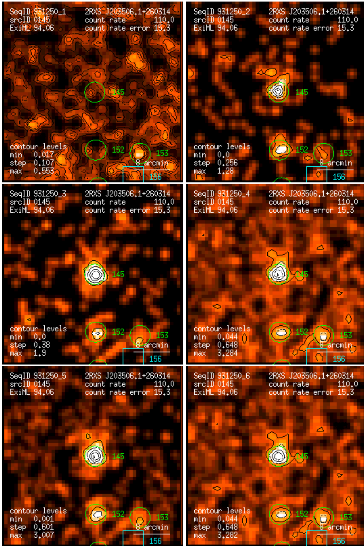
Figure 145: RASS 931250: detection 0145: band rate images, Gaussian filter: (1) PSPC channels 11 – 41, (2) 52 – 90, (3) 91 – 201, (4) 11 – 235, (5) 52 – 201, (6) 11 – 201. Broad band rates in counts/ks. Band rate contour levels in counts/ks/arcmin 2 .
