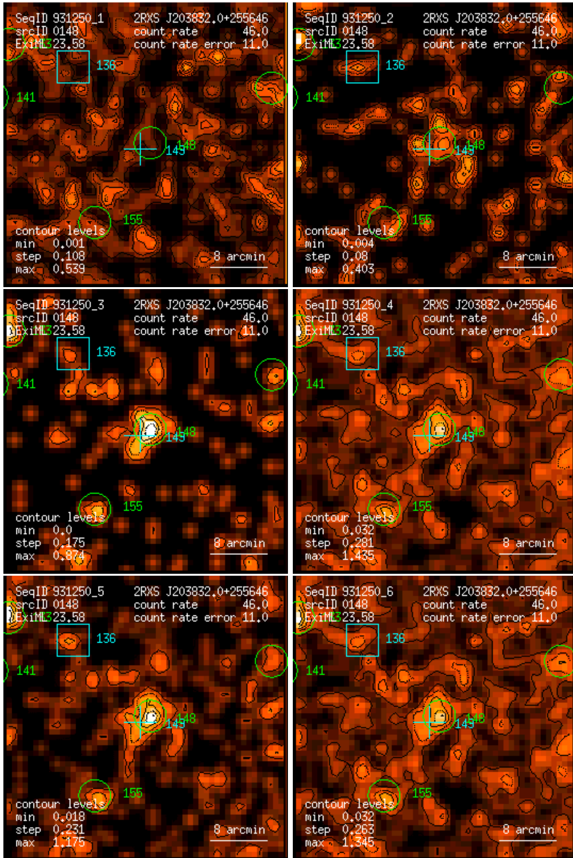
Figure 148: RASS 931250: detection 0148: band rate images, Gaussian filter: (1) PSPC channels 11 – 41, (2) 52 – 90, (3) 91 – 201, (4) 11 – 235, (5) 52 – 201, (6) 11 – 201. Broad band rates in counts/ks. Band rate contour levels in counts/ks/arcmin 2 .
